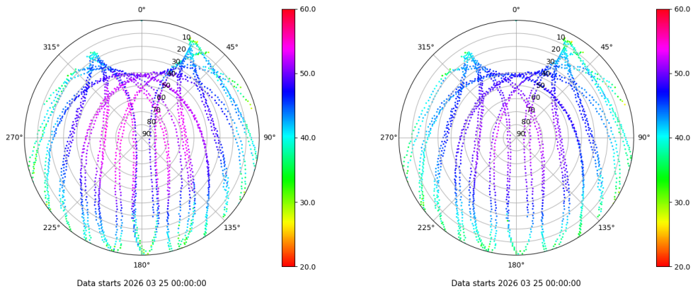
Skyplot for station LRES. Signal to Noise S1C Data file LRES00ESP_R_2026084.xtr Skyplot for station LRES. Signal to Noise S2P Data file LRES00ESP_R_2026084.xtr
