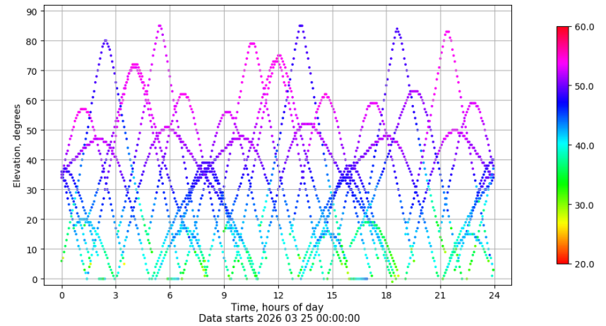
Time-elevation plot for station LRES. Signal to Noise S1C Data file LRES00ESP_R_2026084.xtr
