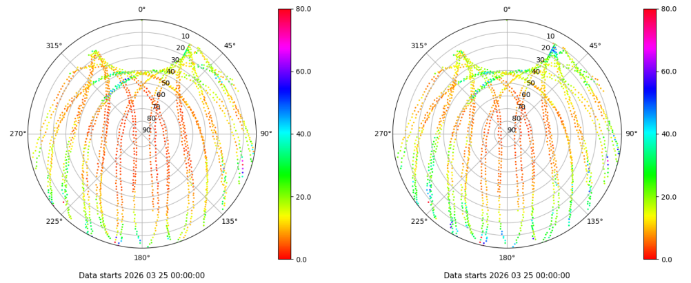
Skyplot for station LRES. Parameter M1C Data file LRES00ESP_R_2026084.xtr Skyplot for station LRES. Parameter M2P Data file LRES00ESP_R_2026084.xtr
