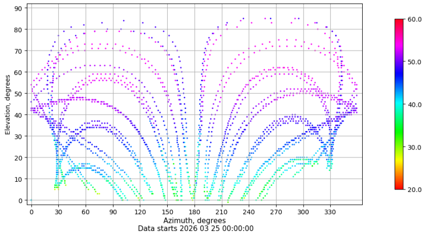
Azimuth-elevation plot for station LRES. Signal to Noise S1C Data file LRES00ESP_R_2026084.xtr
