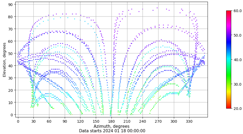
Azimuth-elevation plot for station LRES. Signal to Noise S1C Data file LRES00ESP_R_2024018.xtr
