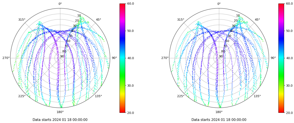
Skyplot for station LRES. Signal to Noise S1C Data file LRES00ESP_R_2024018.xtr Skyplot for station LRES. Signal to Noise S2P Data file LRES00ESP_R_2024018.xtr
