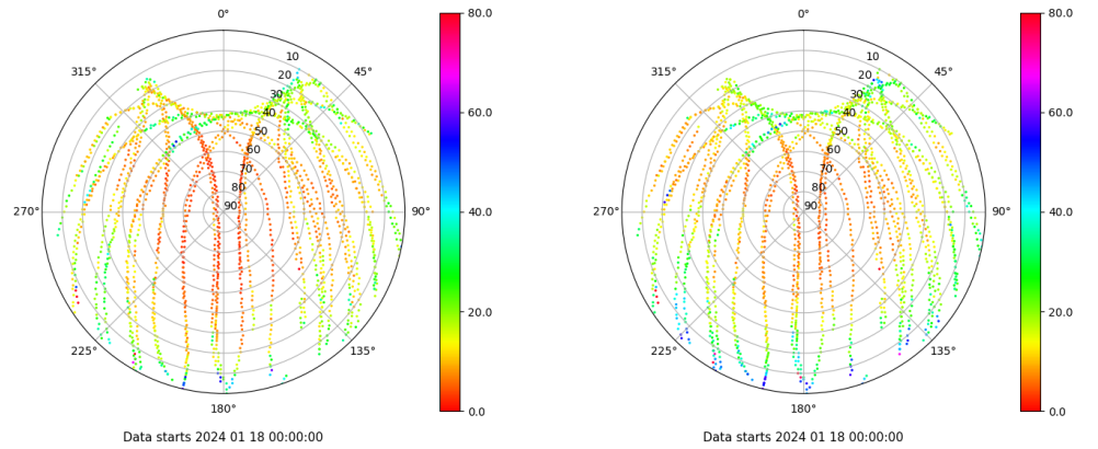
Skyplot for station LRES. Parameter M1C Data file LRES00ESP_R_2024018.xtr Skyplot for station LRES. Parameter M2P Data file LRES00ESP_R_2024018.xtr
