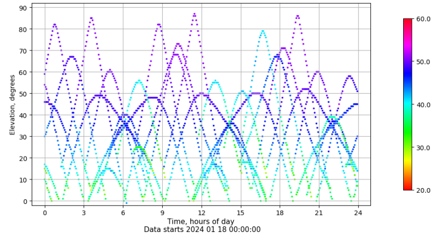
Time-elevation plot for station LRES. Signal to Noise S1C Data file LRES00ESP_R_2024018.xtr
