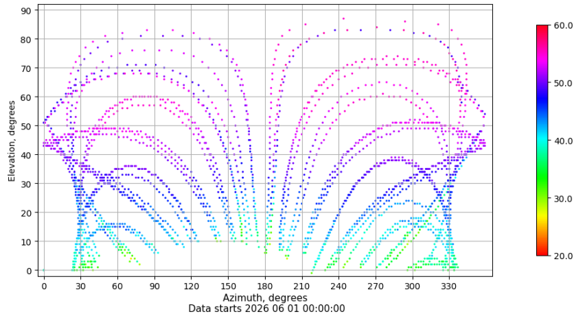
Azimuth-elevation plot for station LPAL. Signal to Noise S1C Data file LPAL00ESP_R_2026152.xtr
