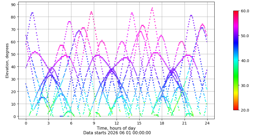
Time-elevation plot for station LPAL. Signal to Noise S1C Data file LPAL00ESP_R_2026152.xtr
