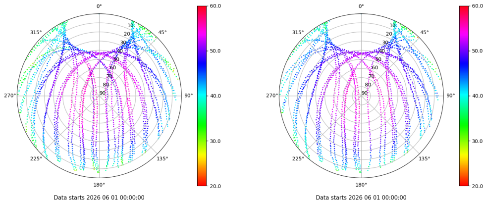
Skyplot for station LPAL. Signal to Noise S1C Data file LPAL00ESP_R_2026152.xtr Skyplot for station LPAL. Signal to Noise S2C Data file LPAL00ESP_R_2026152.xtr
