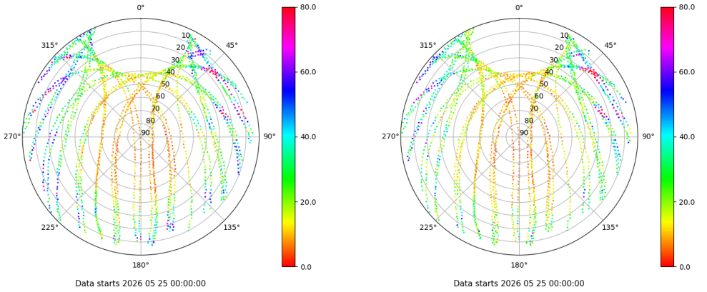
Skyplot for station LPAL. Parameter M1C Data file LPAL00ESP_R_2026145.xtr Skyplot for station LPAL. Parameter M2C Data file LPAL00ESP_R_2026145.xtr
