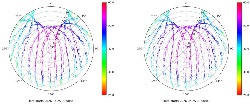
Skyplot for station LPAL. Signal to Noise S1C Data file LPAL00ESP_R_2026145.xtr Skyplot for station LPAL. Signal to Noise S2C Data file LPAL00ESP_R_2026145.xtr
