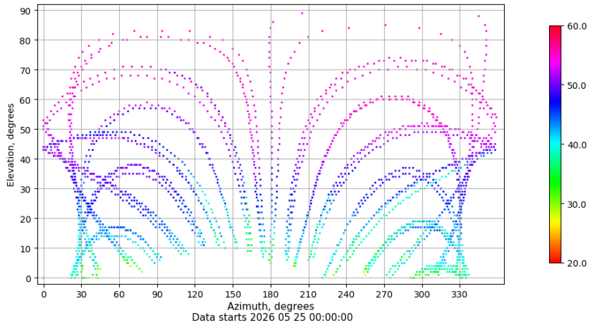
Azimuth-elevation plot for station LPAL. Signal to Noise S1C Data file LPAL00ESP_R_2026145.xtr
