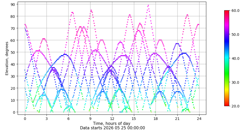
Time-elevation plot for station LPAL. Signal to Noise S1C Data file LPAL00ESP_R_2026145.xtr
