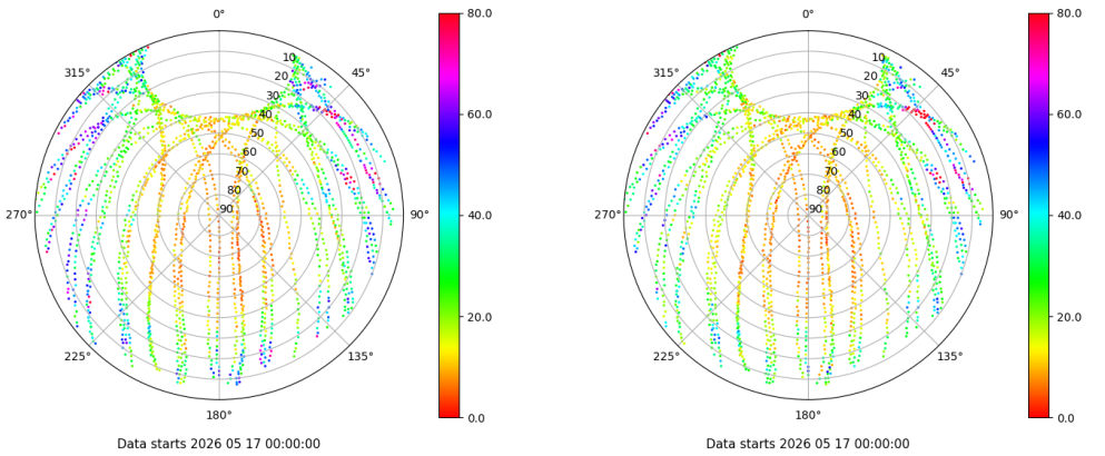
Skyplot for station LPAL. Parameter M1C Data file LPAL00ESP_R_2026137.xtr Skyplot for station LPAL. Parameter M2C Data file LPAL00ESP_R_2026137.xtr
