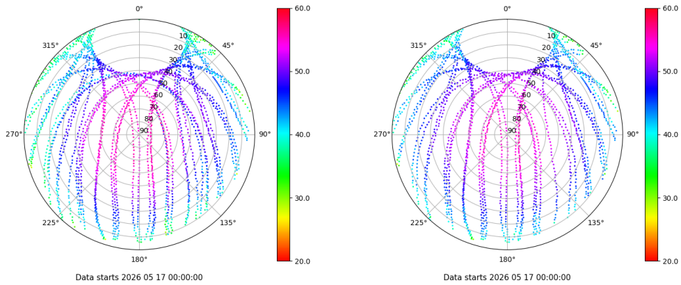
Skyplot for station LPAL. Signal to Noise S1C Data file LPAL00ESP_R_2026137.xtr Skyplot for station LPAL. Signal to Noise S2C Data file LPAL00ESP_R_2026137.xtr
