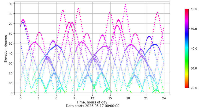
Time-elevation plot for station LPAL. Signal to Noise S1C Data file LPAL00ESP_R_2026137.xtr
