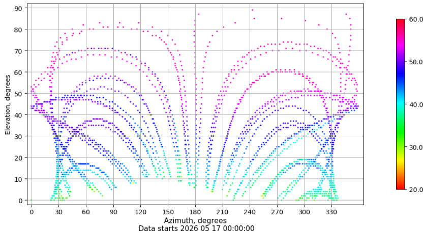
Azimuth-elevation plot for station LPAL. Signal to Noise S1C Data file LPAL00ESP_R_2026137.xtr
