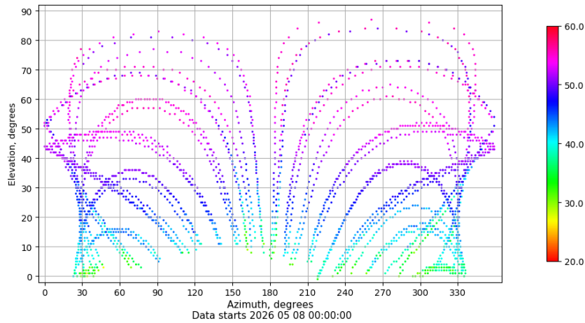
Azimuth-elevation plot for station LPAL. Signal to Noise S1C Data file LPAL00ESP_R_2026128.xtr
