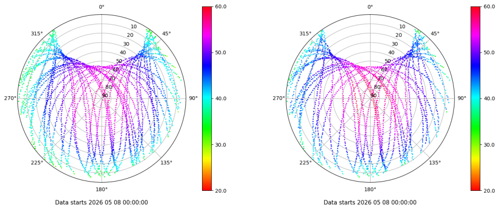
Skyplot for station LPAL. Signal to Noise S1C Data file LPAL00ESP_R_2026128.xtr Skyplot for station LPAL. Signal to Noise S2S Data file LPAL00ESP_R_2026128.xtr
