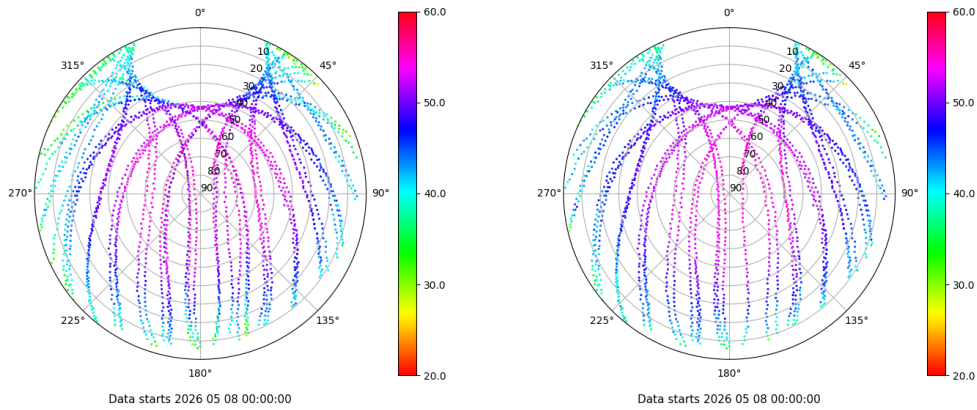
Skyplot for station LPAL. Signal to Noise S1C Data file LPAL00ESP_R_2026128.xtr Skyplot for station LPAL. Signal to Noise S2C Data file LPAL00ESP_R_2026128.xtr
