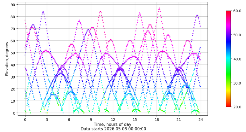
Time-elevation plot for station LPAL. Signal to Noise S1C Data file LPAL00ESP_R_2026128.xtr
