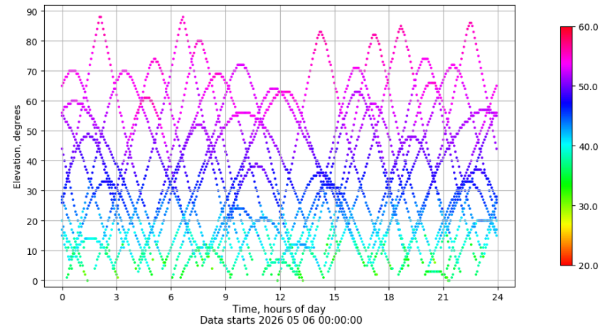
Time-elevation plot for station LPAL. Signal to Noise S1C Data file LPAL00ESP_R_2026126.xtr
