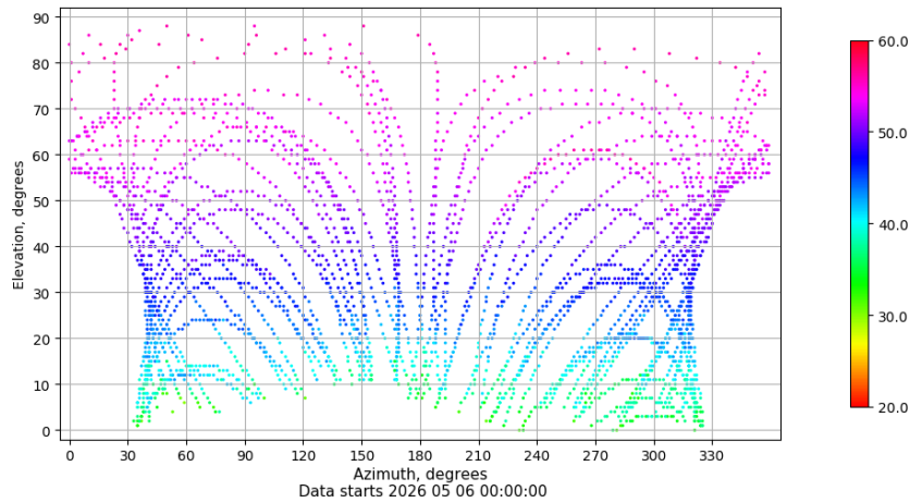
Azimuth-elevation plot for station LPAL. Signal to Noise S1C Data file LPAL00ESP_R_2026126.xtr
