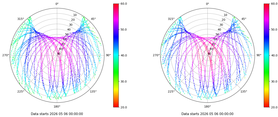
Skyplot for station LPAL. Signal to Noise S1C Data file LPAL00ESP_R_2026126.xtr Skyplot for station LPAL. Signal to Noise S2S Data file LPAL00ESP_R_2026126.xtr
