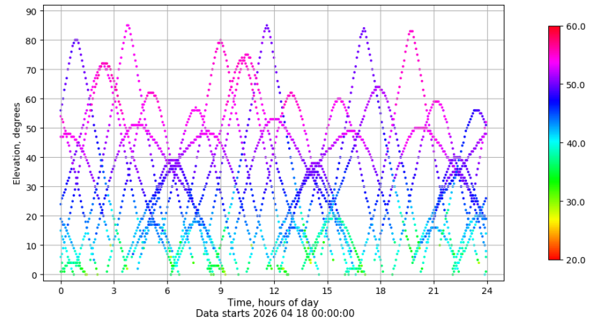
Time-elevation plot for station LPAL. Signal to Noise S1C Data file LPAL00ESP_R_2026108.xtr
