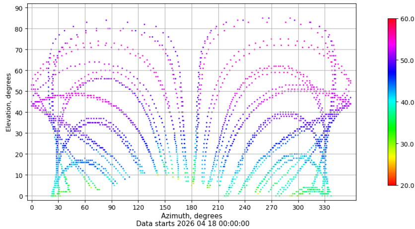
Azimuth-elevation plot for station LPAL. Signal to Noise S1C Data file LPAL00ESP_R_2026108.xtr
