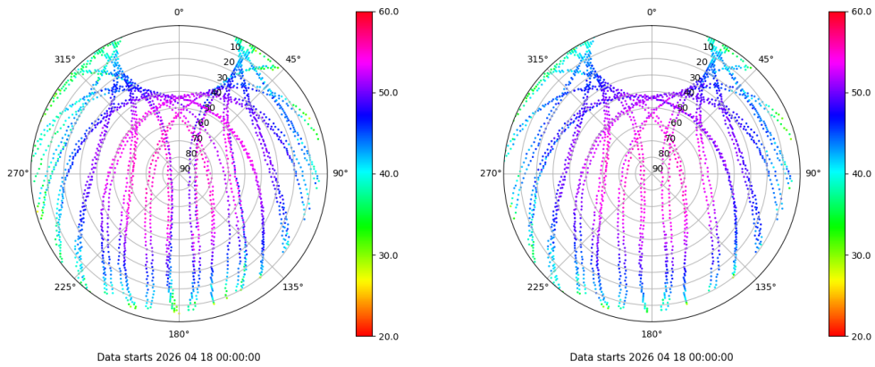
Skyplot for station LPAL. Signal to Noise S1C Data file LPAL00ESP_R_2026108.xtr Skyplot for station LPAL. Signal to Noise S2C Data file LPAL00ESP_R_2026108.xtr
