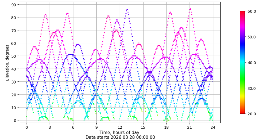
Time-elevation plot for station LPAL. Signal to Noise S1C Data file LPAL00ESP_R_2026087.xtr
