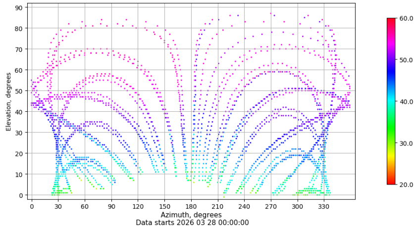
Azimuth-elevation plot for station LPAL. Signal to Noise S1C Data file LPAL00ESP_R_2026087.xtr
