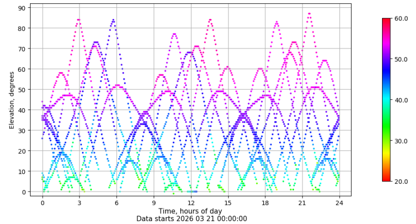
Time-elevation plot for station LPAL. Signal to Noise S1C Data file LPAL00ESP_R_2026080.xtr
