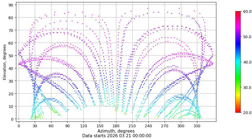
Azimuth-elevation plot for station LPAL. Signal to Noise S1C Data file LPAL00ESP_R_2026080.xtr
