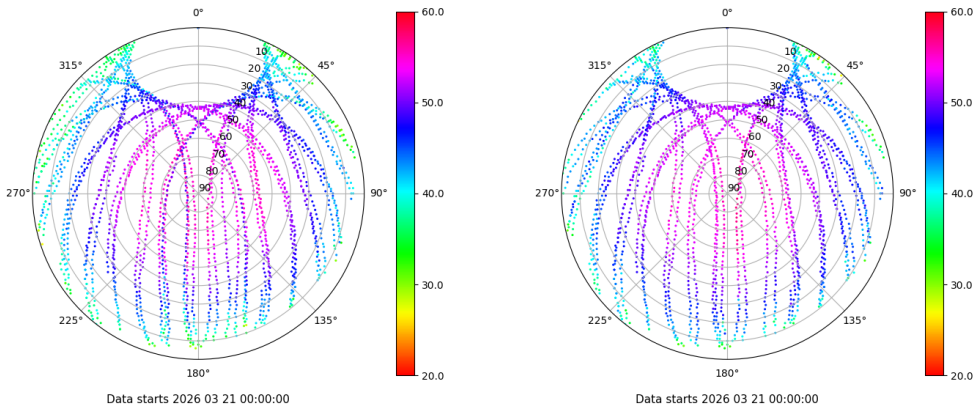
Skyplot for station LPAL. Signal to Noise S1C Data file LPAL00ESP_R_2026080.xtr Skyplot for station LPAL. Signal to Noise S2C Data file LPAL00ESP_R_2026080.xtr
