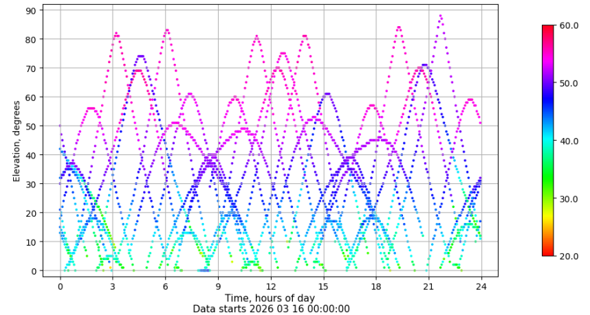
Time-elevation plot for station LPAL. Signal to Noise S1C Data file LPAL00ESP_R_2026075.xtr
