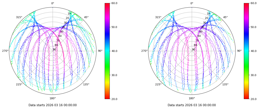
Skyplot for station LPAL. Signal to Noise S1C Data file LPAL00ESP_R_2026075.xtr Skyplot for station LPAL. Signal to Noise S2C Data file LPAL00ESP_R_2026075.xtr
