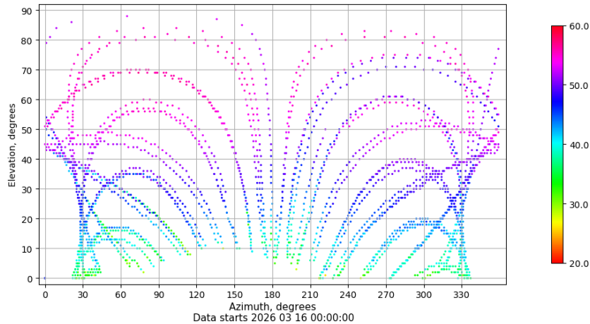
Azimuth-elevation plot for station LPAL. Signal to Noise S1C Data file LPAL00ESP_R_2026075.xtr
