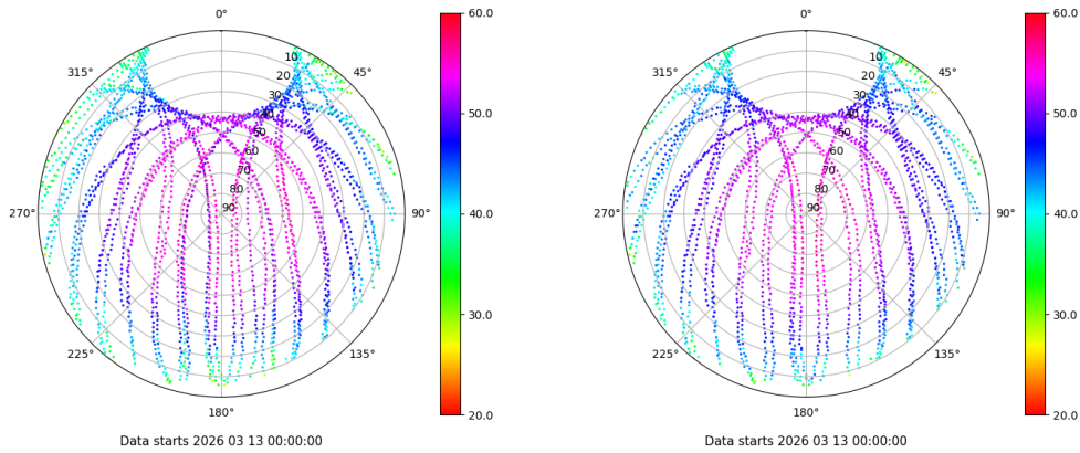
Skyplot for station LPAL. Signal to Noise S1C Data file LPAL00ESP_R_2026072.xtr Skyplot for station LPAL. Signal to Noise S2C Data file LPAL00ESP_R_2026072.xtr
