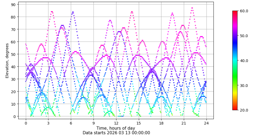
Time-elevation plot for station LPAL. Signal to Noise S1C Data file LPAL00ESP_R_2026072.xtr
