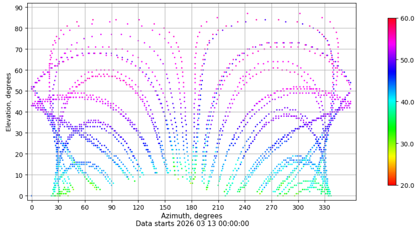
Azimuth-elevation plot for station LPAL. Signal to Noise S1C Data file LPAL00ESP_R_2026072.xtr
