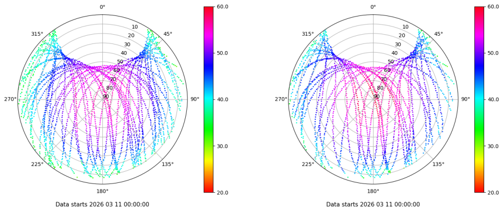
Skyplot for station LPAL. Signal to Noise S1C Data file LPAL00ESP_R_2026070.xtr Skyplot for station LPAL. Signal to Noise S2S Data file LPAL00ESP_R_2026070.xtr
