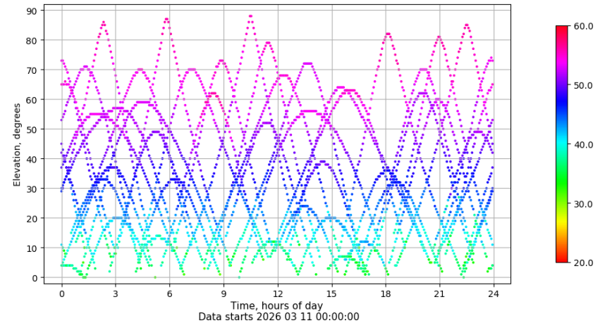
Time-elevation plot for station LPAL. Signal to Noise S1C Data file LPAL00ESP_R_2026070.xtr
