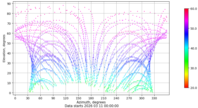
Azimuth-elevation plot for station LPAL. Signal to Noise S1C Data file LPAL00ESP_R_2026070.xtr
