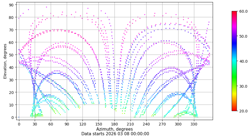
Azimuth-elevation plot for station LPAL. Signal to Noise S1C Data file LPAL00ESP_R_2026067.xtr
