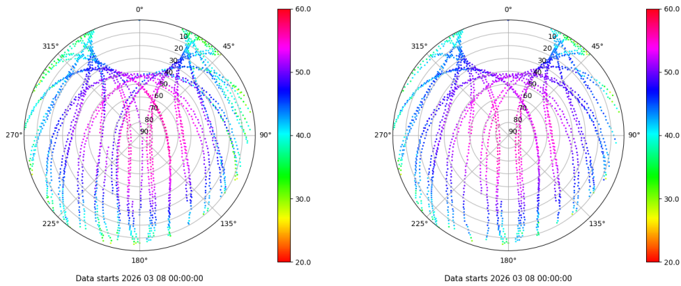
Skyplot for station LPAL. Signal to Noise S1C Data file LPAL00ESP_R_2026067.xtr Skyplot for station LPAL. Signal to Noise S2C Data file LPAL00ESP_R_2026067.xtr
