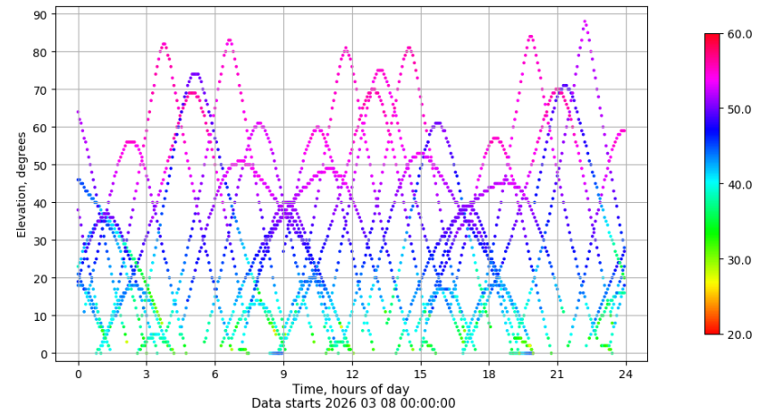
Time-elevation plot for station LPAL. Signal to Noise S1C Data file LPAL00ESP_R_2026067.xtr
