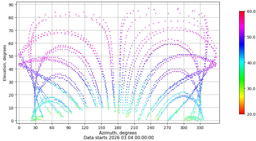
Azimuth-elevation plot for station LPAL. Signal to Noise S1C Data file LPAL00ESP_R_2026063.xtr
