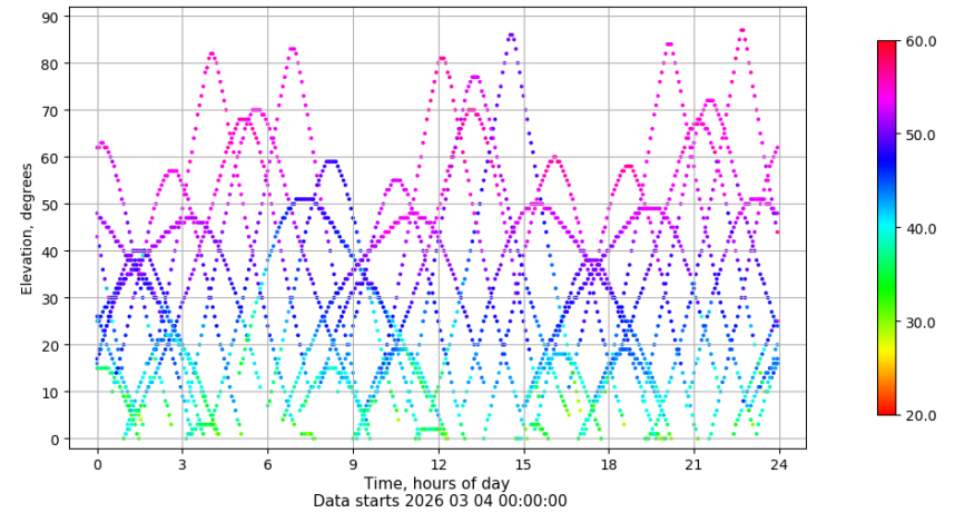
Time-elevation plot for station LPAL. Signal to Noise S1C Data file LPAL00ESP_R_2026063.xtr
