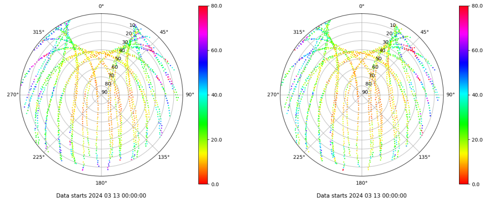
Skyplot for station LPAL. Parameter M1C Data file LPAL00ESP_R_2024073.xtr Skyplot for station LPAL. Parameter M2C Data file LPAL00ESP_R_2024073.xtr
