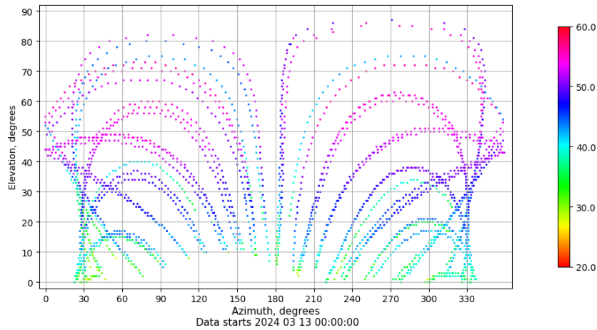
Azimuth-elevation plot for station LPAL. Signal to Noise S1C Data file LPAL00ESP_R_2024073.xtr
