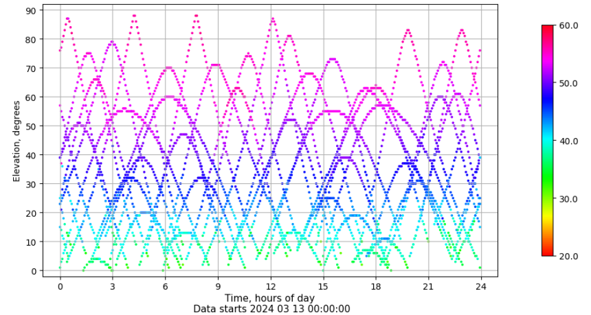
Time-elevation plot for station LPAL. Signal to Noise S1C Data file LPAL00ESP_R_2024073.xtr
