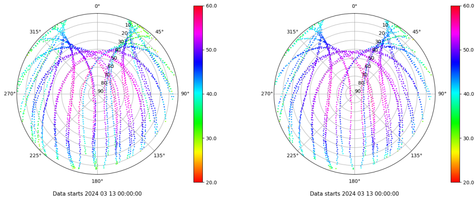
Skyplot for station LPAL. Signal to Noise S1C Data file LPAL00ESP_R_2024073.xtr Skyplot for station LPAL. Signal to Noise S2C Data file LPAL00ESP_R_2024073.xtr
