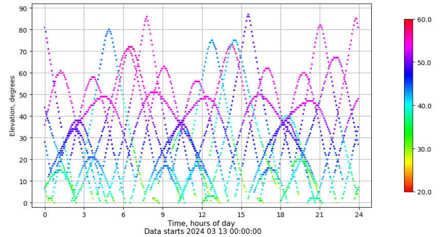
Time-elevation plot for station LPAL. Signal to Noise S1C Data file LPAL00ESP_R_2024073.xtr
