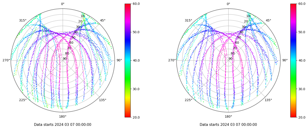
Skyplot for station LPAL. Signal to Noise S1C Data file LPAL00ESP_R_2024067.xtr Skyplot for station LPAL. Signal to Noise S2C Data file LPAL00ESP_R_2024067.xtr
