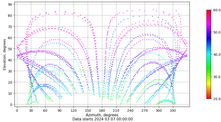
Azimuth-elevation plot for station LPAL. Signal to Noise S1C Data file LPAL00ESP_R_2024067.xtr
