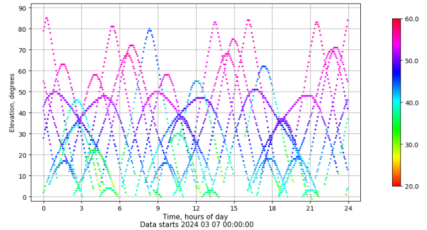
Time-elevation plot for station LPAL. Signal to Noise S1C Data file LPAL00ESP_R_2024067.xtr
