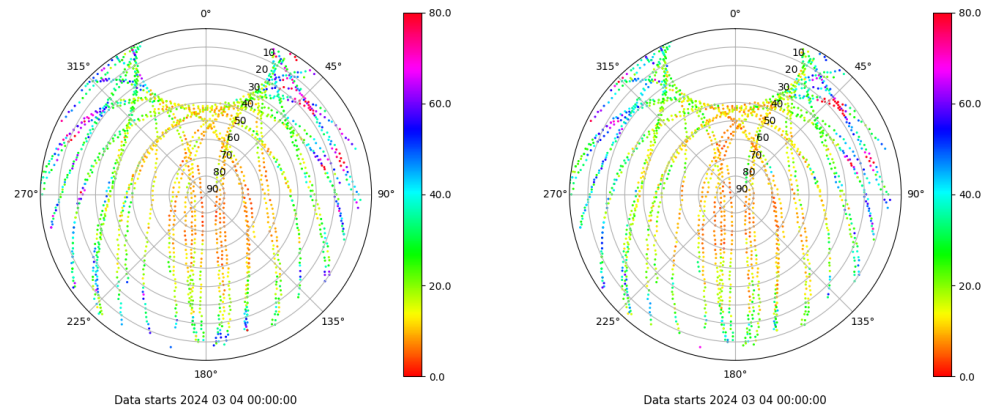
Skyplot for station LPAL. Parameter M1C Data file LPAL00ESP_R_2024064.xtr Skyplot for station LPAL. Parameter M2C Data file LPAL00ESP_R_2024064.xtr
