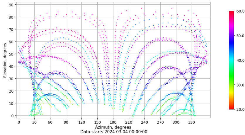
Azimuth-elevation plot for station LPAL. Signal to Noise S1C Data file LPAL00ESP_R_2024064.xtr
