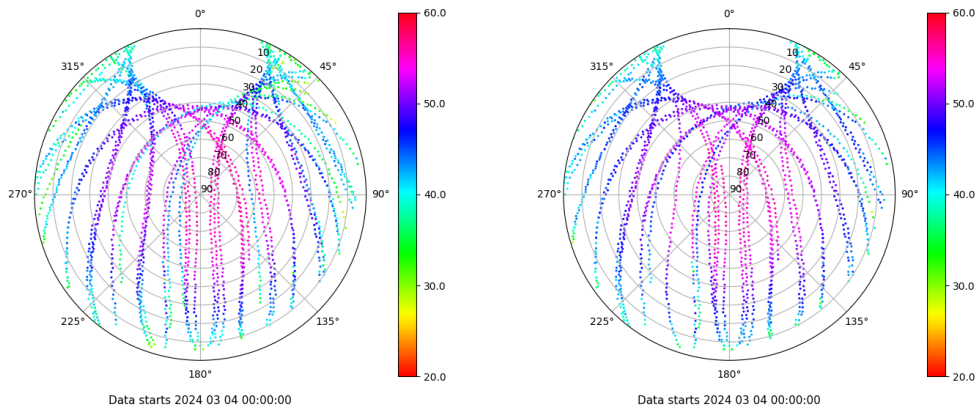
Skyplot for station LPAL. Signal to Noise S1C Data file LPAL00ESP_R_2024064.xtr Skyplot for station LPAL. Signal to Noise S2C Data file LPAL00ESP_R_2024064.xtr
