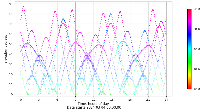
Time-elevation plot for station LPAL. Signal to Noise S1C Data file LPAL00ESP_R_2024064.xtr
