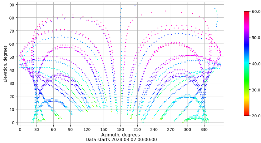
Azimuth-elevation plot for station LPAL. Signal to Noise S1C Data file LPAL00ESP_R_2024062.xtr
