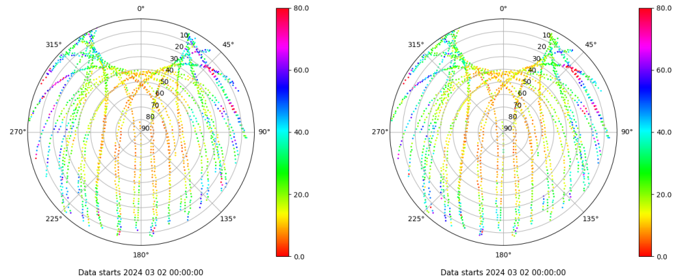
Skyplot for station LPAL. Parameter M1C Data file LPAL00ESP_R_2024062.xtr Skyplot for station LPAL. Parameter M2C Data file LPAL00ESP_R_2024062.xtr
