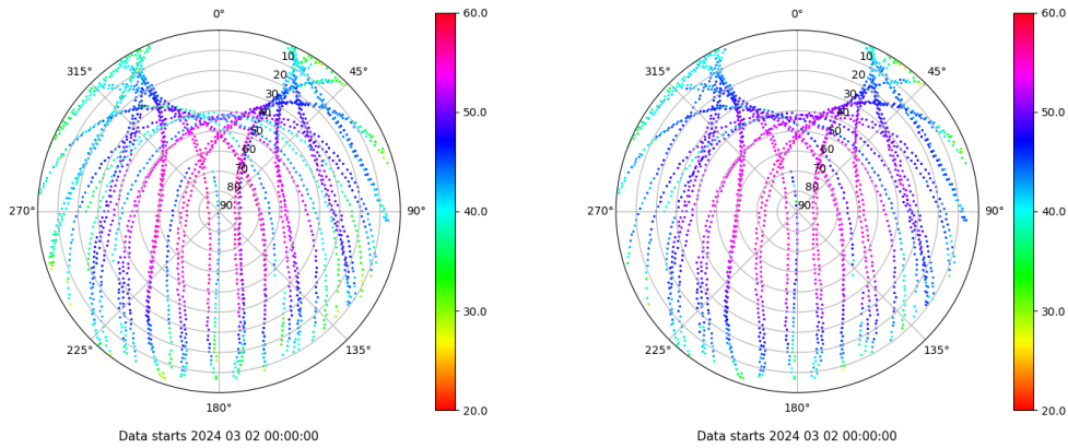
Skyplot for station LPAL. Signal to Noise S1C Data file LPAL00ESP_R_2024062.xtr Skyplot for station LPAL. Signal to Noise S2C Data file LPAL00ESP_R_2024062.xtr
