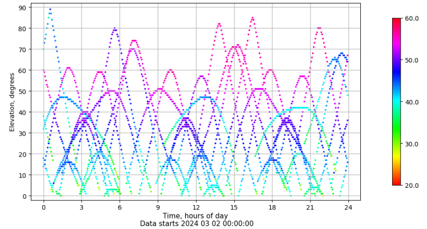
Time-elevation plot for station LPAL. Signal to Noise S1C Data file LPAL00ESP_R_2024062.xtr
