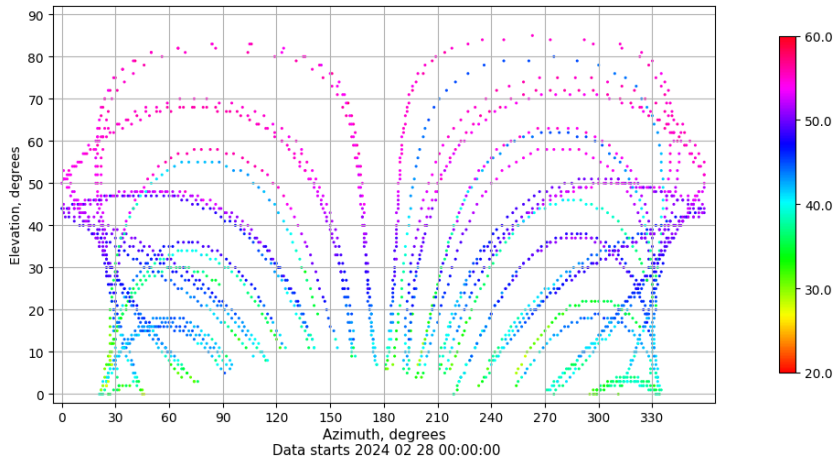
Azimuth-elevation plot for station LPAL. Signal to Noise S1C Data file LPAL00ESP_R_2024059.xtr
