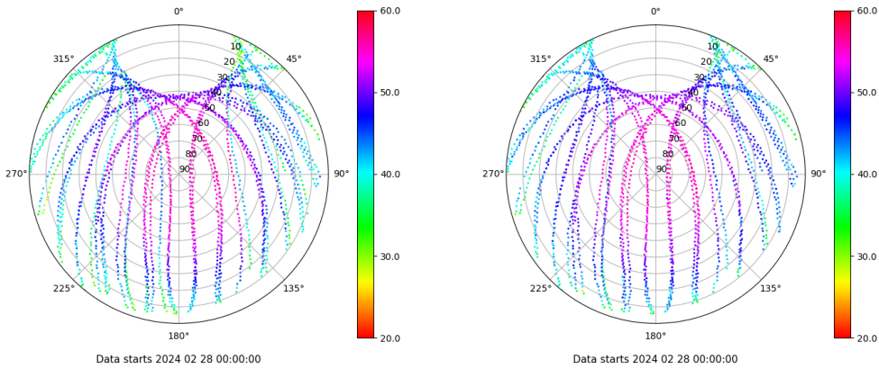
Skyplot for station LPAL. Signal to Noise S1C Data file LPAL00ESP_R_2024059.xtr Skyplot for station LPAL. Signal to Noise S2C Data file LPAL00ESP_R_2024059.xtr
