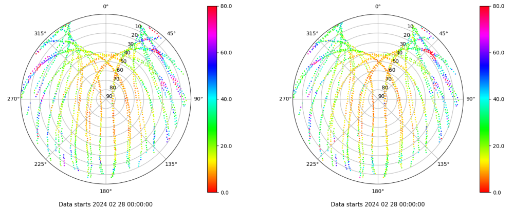
Skyplot for station LPAL. Parameter M1C Data file LPAL00ESP_R_2024059.xtr Skyplot for station LPAL. Parameter M2C Data file LPAL00ESP_R_2024059.xtr
