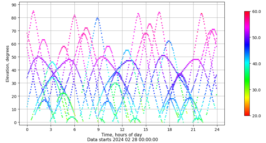
Time-elevation plot for station LPAL. Signal to Noise S1C Data file LPAL00ESP_R_2024059.xtr
