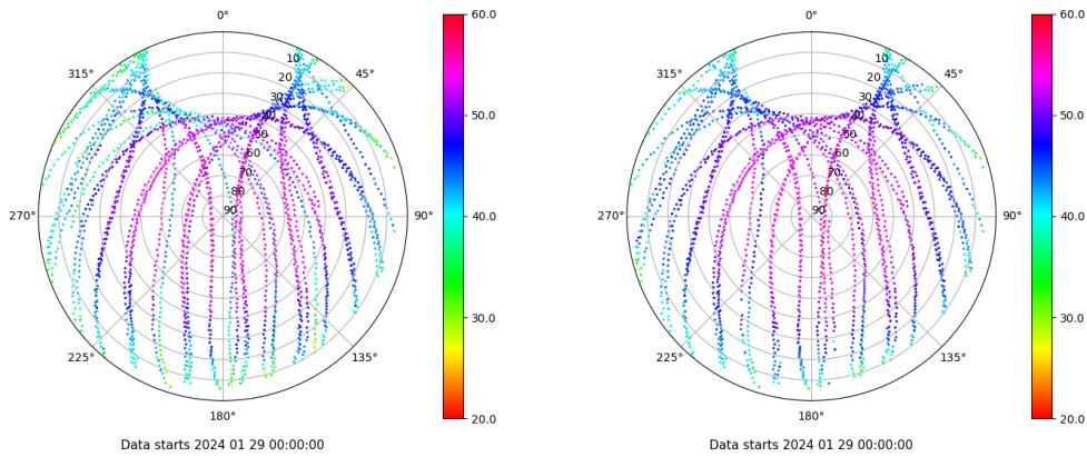
Skyplot for station LPAL. Signal to Noise S1C Data file LPAL00ESP_R_2024029.xtr Skyplot for station LPAL. Signal to Noise S2C Data file LPAL00ESP_R_2024029.xtr
