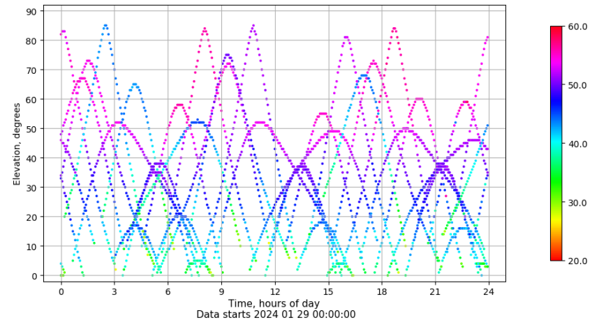
Time-elevation plot for station LPAL. Signal to Noise S1C Data file LPAL00ESP_R_2024029.xtr
