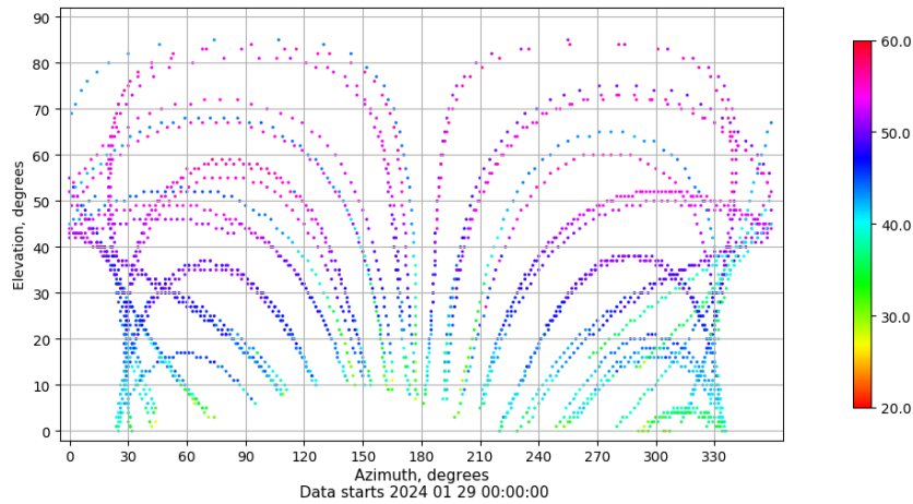
Azimuth-elevation plot for station LPAL. Signal to Noise S1C Data file LPAL00ESP_R_2024029.xtr
