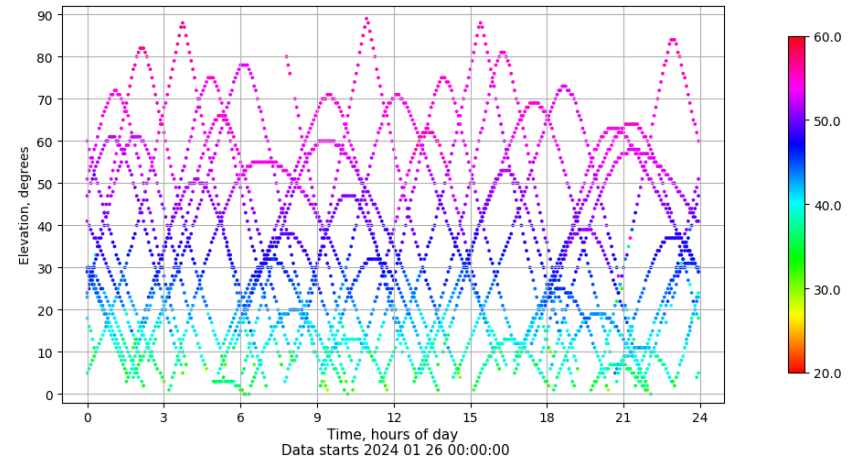
Time-elevation plot for station LPAL. Signal to Noise S1C Data file LPAL00ESP_R_2024026.xtr
