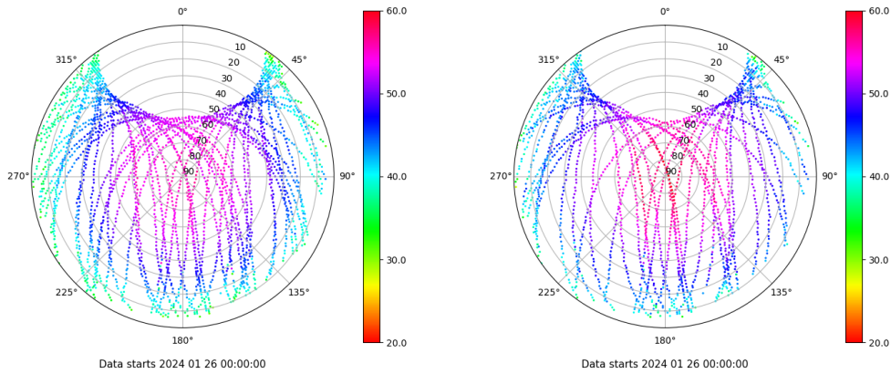
Skyplot for station LPAL. Signal to Noise S1C Data file LPAL00ESP_R_2024026.xtr Skyplot for station LPAL. Signal to Noise S2S Data file LPAL00ESP_R_2024026.xtr
