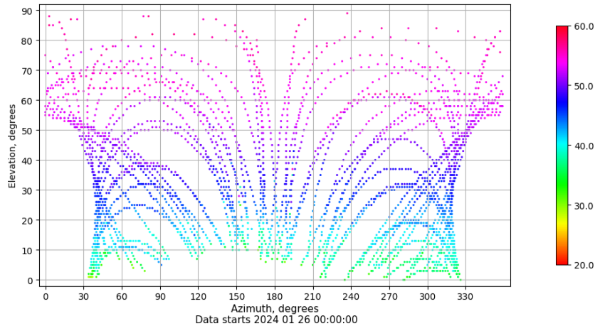
Azimuth-elevation plot for station LPAL. Signal to Noise S1C Data file LPAL00ESP_R_2024026.xtr
