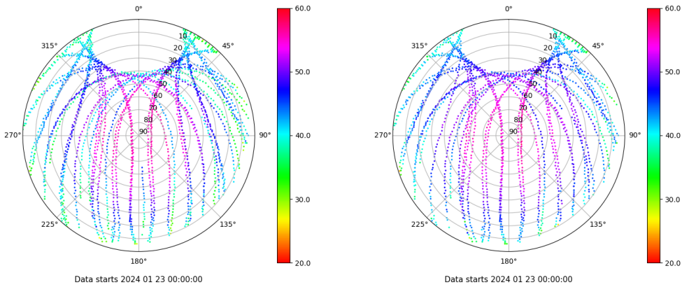
Skyplot for station LPAL. Signal to Noise S1C Data file LPAL00ESP_R_2024023.xtr Skyplot for station LPAL. Signal to Noise S2C Data file LPAL00ESP_R_2024023.xtr
