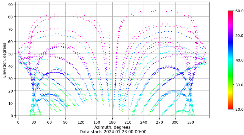
Azimuth-elevation plot for station LPAL. Signal to Noise S1C Data file LPAL00ESP_R_2024023.xtr
