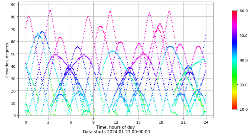
Time-elevation plot for station LPAL. Signal to Noise S1C Data file LPAL00ESP_R_2024023.xtr
