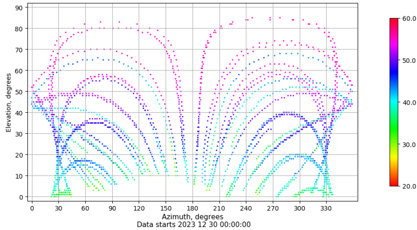
Azimuth-elevation plot for station LPAL. Signal to Noise S1C Data file LPAL00ESP_R_2023364.xtr
