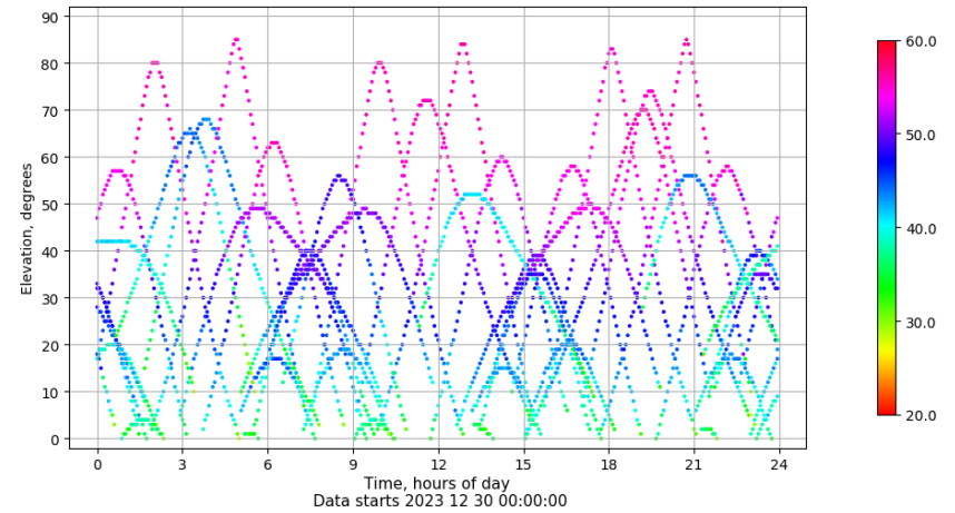
Time-elevation plot for station LPAL. Signal to Noise S1C Data file LPAL00ESP_R_2023364.xtr
