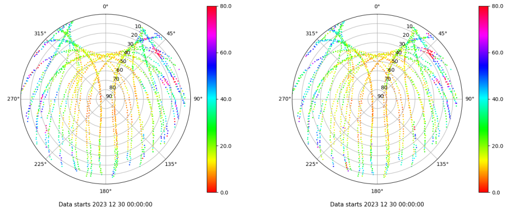
Skyplot for station LPAL. Parameter M1C Data file LPAL00ESP_R_2023364.xtr Skyplot for station LPAL. Parameter M2C Data file LPAL00ESP_R_2023364.xtr
