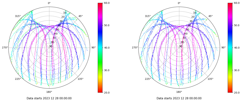
Skyplot for station LPAL. Signal to Noise S1C Data file LPAL00ESP_R_2023362.xtr Skyplot for station LPAL. Signal to Noise S2C Data file LPAL00ESP_R_2023362.xtr
