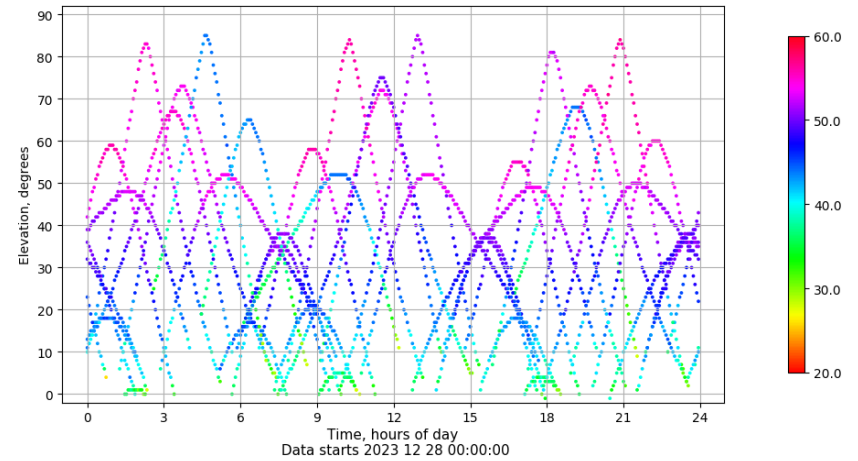
Time-elevation plot for station LPAL. Signal to Noise S1C Data file LPAL00ESP_R_2023362.xtr
