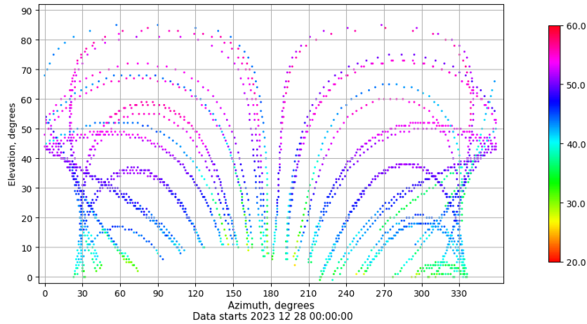
Azimuth-elevation plot for station LPAL. Signal to Noise S1C Data file LPAL00ESP_R_2023362.xtr
