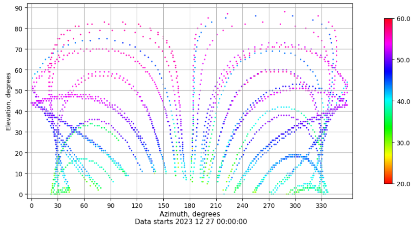
Azimuth-elevation plot for station LPAL. Signal to Noise S1C Data file LPAL00ESP_R_2023361.xtr
