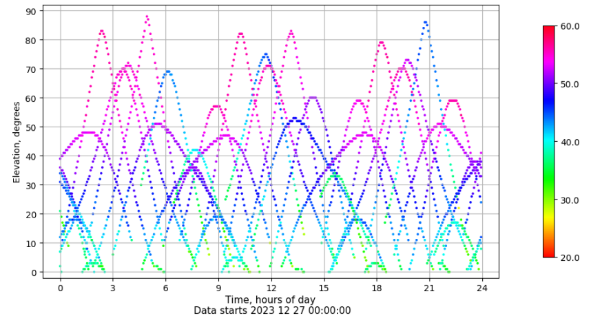
Time-elevation plot for station LPAL. Signal to Noise S1C Data file LPAL00ESP_R_2023361.xtr
