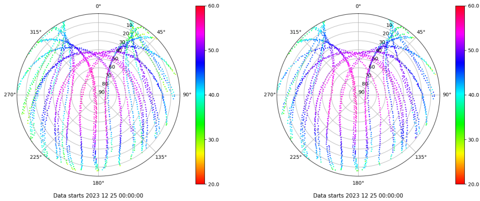
Skyplot for station LPAL. Signal to Noise S1C Data file LPAL00ESP_R_2023359.xtr Skyplot for station LPAL. Signal to Noise S2C Data file LPAL00ESP_R_2023359.xtr
