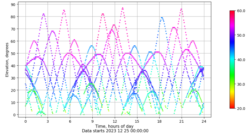
Time-elevation plot for station LPAL. Signal to Noise S1C Data file LPAL00ESP_R_2023359.xtr
