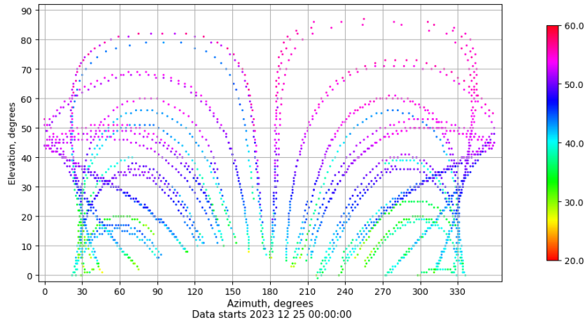
Azimuth-elevation plot for station LPAL. Signal to Noise S1C Data file LPAL00ESP_R_2023359.xtr
