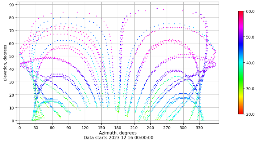
Azimuth-elevation plot for station LPAL. Signal to Noise S1C Data file LPAL00ESP_R_2023350.xtr
