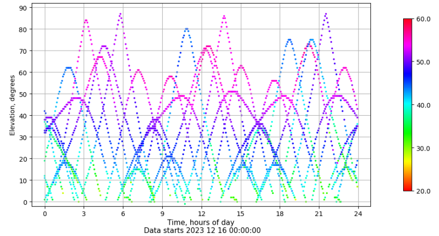
Time-elevation plot for station LPAL. Signal to Noise S1C Data file LPAL00ESP_R_2023350.xtr
