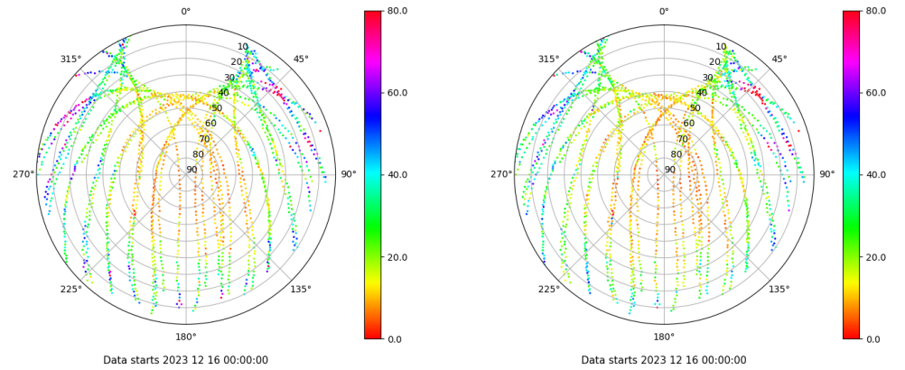
Skyplot for station LPAL. Parameter M1C Data file LPAL00ESP_R_2023350.xtr Skyplot for station LPAL. Parameter M2C Data file LPAL00ESP_R_2023350.xtr
