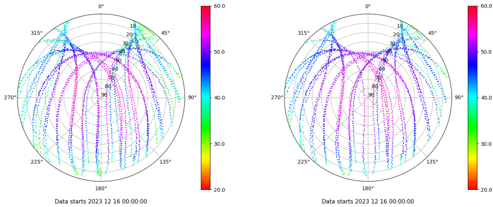
Skyplot for station LPAL. Signal to Noise S1C Data file LPAL00ESP_R_2023350.xtr Skyplot for station LPAL. Signal to Noise S2C Data file LPAL00ESP_R_2023350.xtr
