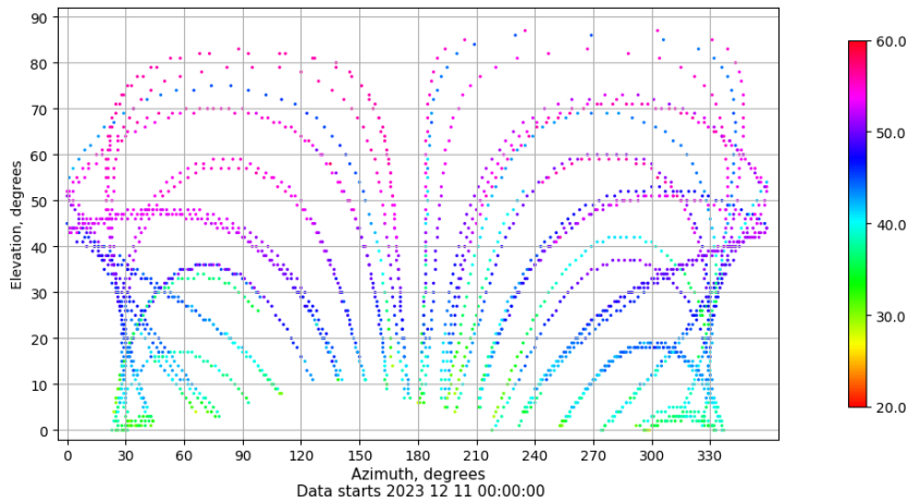
Azimuth-elevation plot for station LPAL. Signal to Noise S1C Data file LPAL00ESP_R_2023345.xtr
