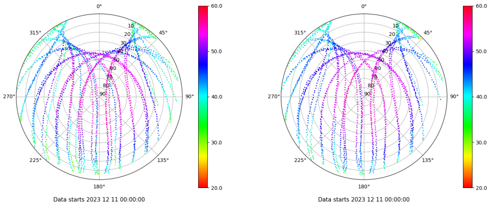
Skyplot for station LPAL. Signal to Noise S1C Data file LPAL00ESP_R_2023345.xtr Skyplot for station LPAL. Signal to Noise S2C Data file LPAL00ESP_R_2023345.xtr
