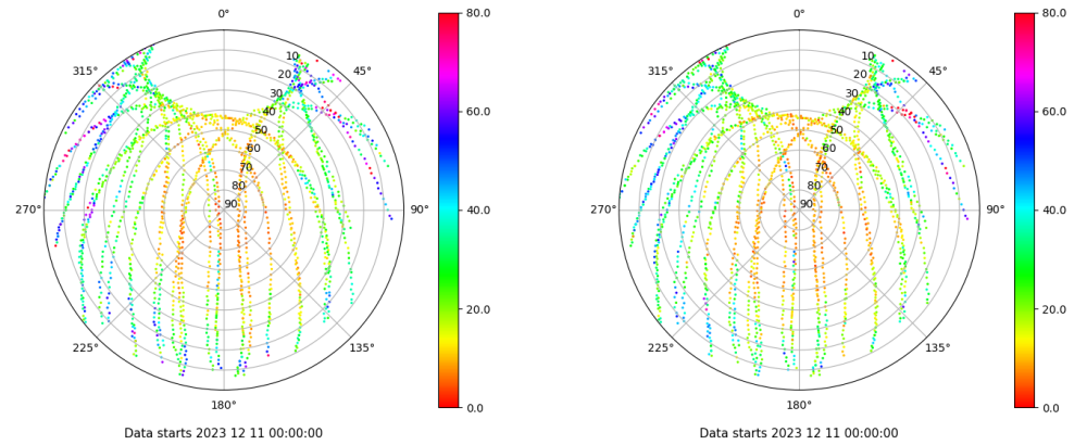
Skyplot for station LPAL. Parameter M1C Data file LPAL00ESP_R_2023345.xtr Skyplot for station LPAL. Parameter M2C Data file LPAL00ESP_R_2023345.xtr
