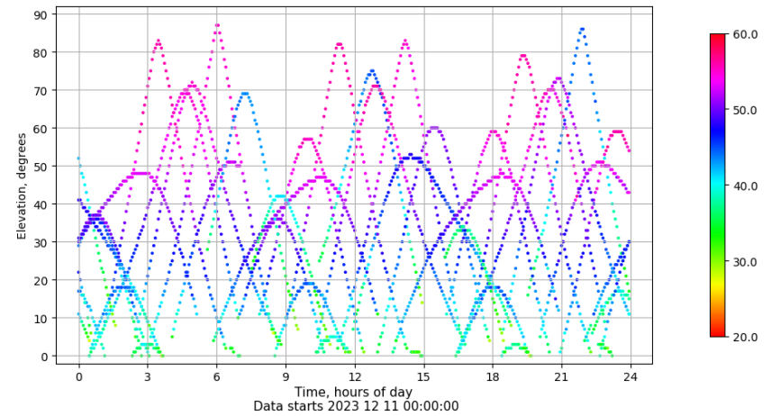
Time-elevation plot for station LPAL. Signal to Noise S1C Data file LPAL00ESP_R_2023345.xtr
