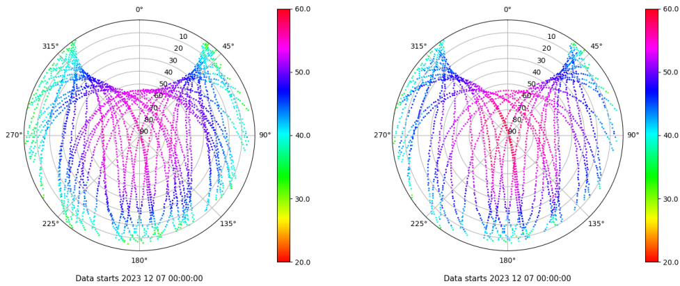
Skyplot for station LPAL. Signal to Noise S1C Data file LPAL00ESP_R_2023341.xtr Skyplot for station LPAL. Signal to Noise S2S Data file LPAL00ESP_R_2023341.xtr
