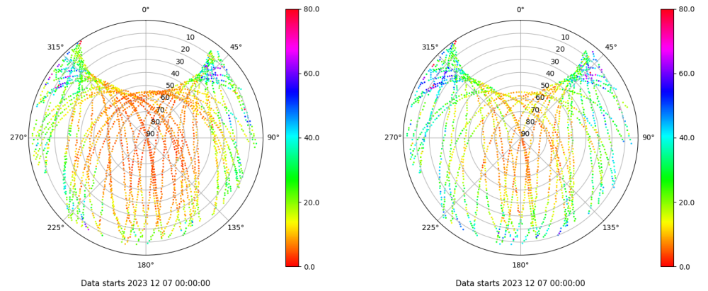
Skyplot for station LPAL. Parameter M1C Data file LPAL00ESP_R_2023341.xtr Skyplot for station LPAL. Parameter M2S Data file LPAL00ESP_R_2023341.xtr
