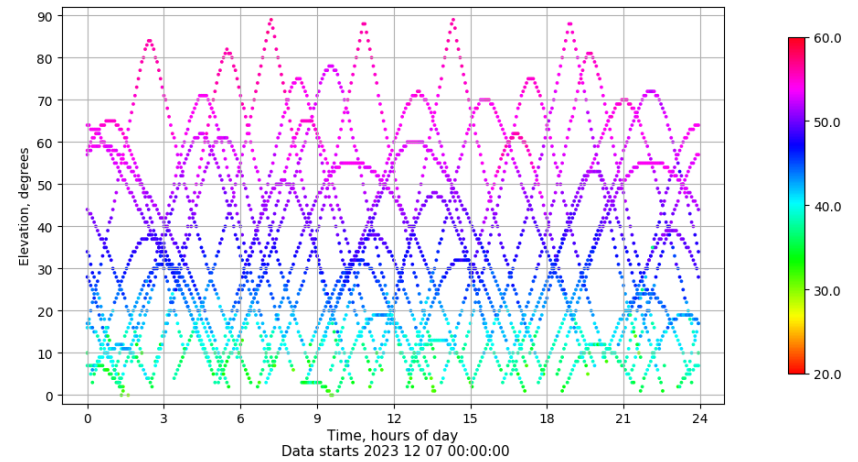
Time-elevation plot for station LPAL. Signal to Noise S1C Data file LPAL00ESP_R_2023341.xtr
