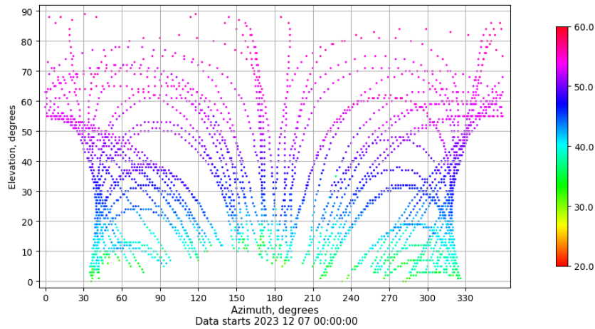
Azimuth-elevation plot for station LPAL. Signal to Noise S1C Data file LPAL00ESP_R_2023341.xtr
