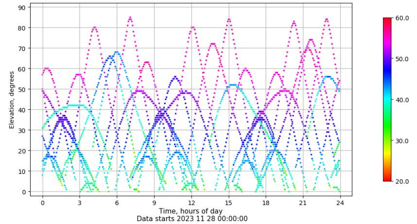
Time-elevation plot for station LPAL. Signal to Noise S1C Data file LPAL00ESP_R_2023332.xtr
