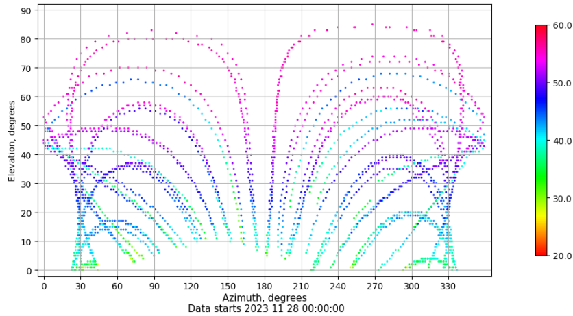
Azimuth-elevation plot for station LPAL. Signal to Noise S1C Data file LPAL00ESP_R_2023332.xtr
