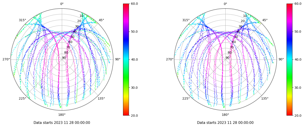
Skyplot for station LPAL. Signal to Noise S1C Data file LPAL00ESP_R_2023332.xtr Skyplot for station LPAL. Signal to Noise S2C Data file LPAL00ESP_R_2023332.xtr
