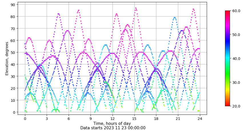
Time-elevation plot for station LPAL. Signal to Noise S1C Data file LPAL00ESP_R_2023327.xtr
