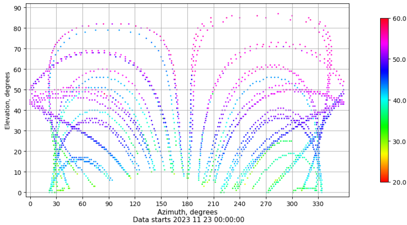
Azimuth-elevation plot for station LPAL. Signal to Noise S1C Data file LPAL00ESP_R_2023327.xtr
