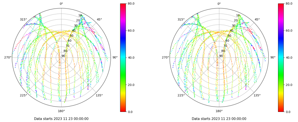
Skyplot for station LPAL. Parameter M1C Data file LPAL00ESP_R_2023327.xtr Skyplot for station LPAL. Parameter M2C Data file LPAL00ESP_R_2023327.xtr
