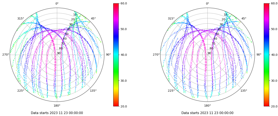
Skyplot for station LPAL. Signal to Noise S1C Data file LPAL00ESP_R_2023327.xtr Skyplot for station LPAL. Signal to Noise S2C Data file LPAL00ESP_R_2023327.xtr
