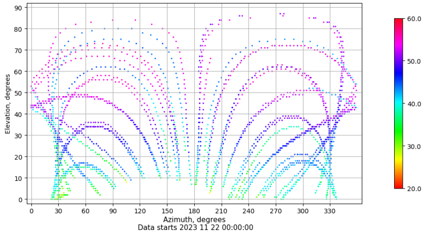
Azimuth-elevation plot for station LPAL. Signal to Noise S1C Data file LPAL00ESP_R_2023326.xtr
