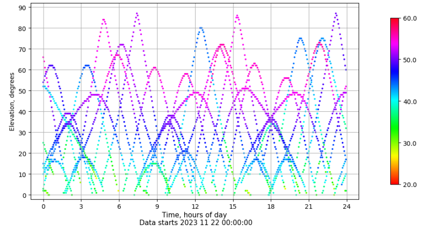
Time-elevation plot for station LPAL. Signal to Noise S1C Data file LPAL00ESP_R_2023326.xtr
