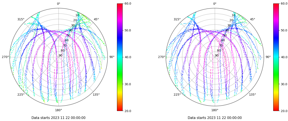
Skyplot for station LPAL. Signal to Noise S1C Data file LPAL00ESP_R_2023326.xtr Skyplot for station LPAL. Signal to Noise S2C Data file LPAL00ESP_R_2023326.xtr
