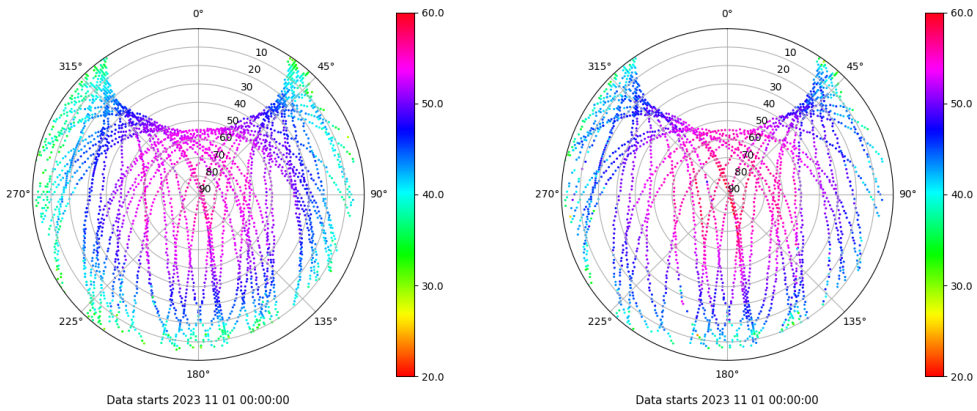
Skyplot for station LPAL. Signal to Noise S1C Data file LPAL00ESP_R_2023305.xtr Skyplot for station LPAL. Signal to Noise S2S Data file LPAL00ESP_R_2023305.xtr
