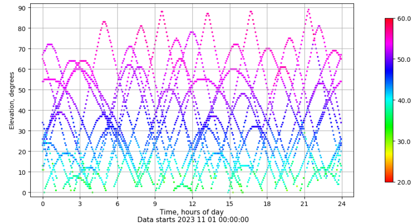
Time-elevation plot for station LPAL. Signal to Noise S1C Data file LPAL00ESP_R_2023305.xtr
