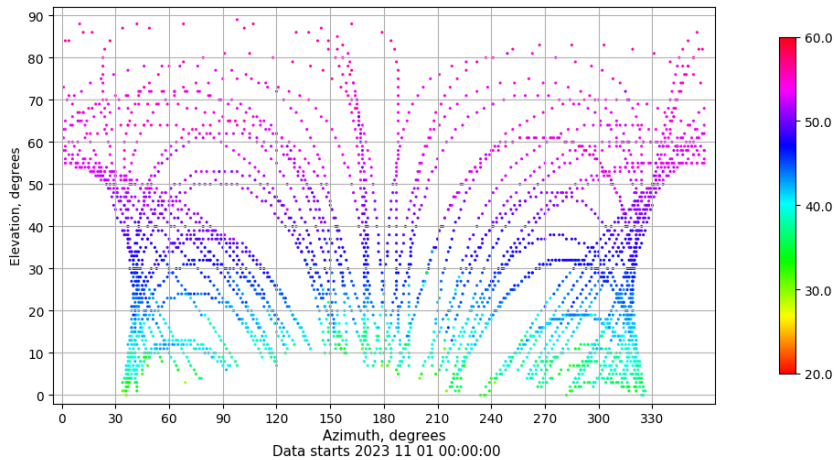
Azimuth-elevation plot for station LPAL. Signal to Noise S1C Data file LPAL00ESP_R_2023305.xtr
