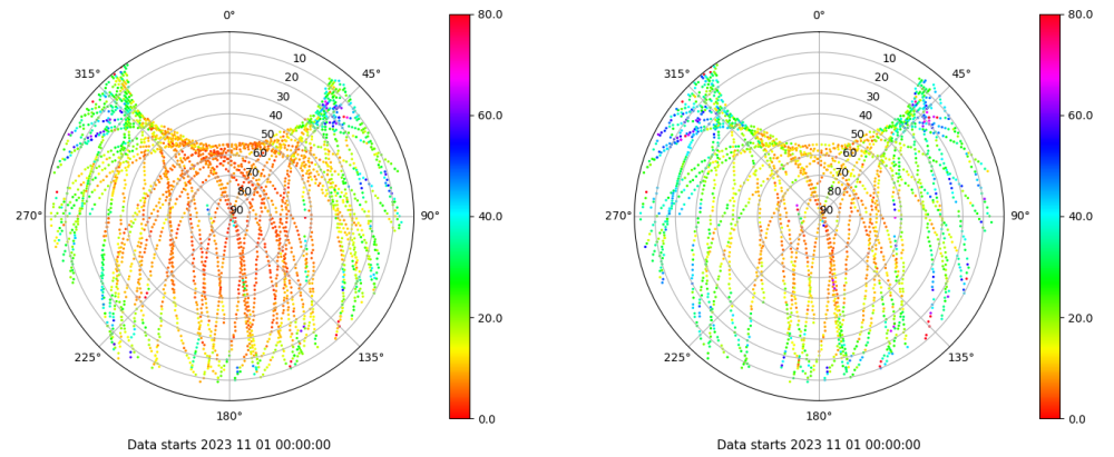
Skyplot for station LPAL. Parameter M1C Data file LPAL00ESP_R_2023305.xtr Skyplot for station LPAL. Parameter M2S Data file LPAL00ESP_R_2023305.xtr
