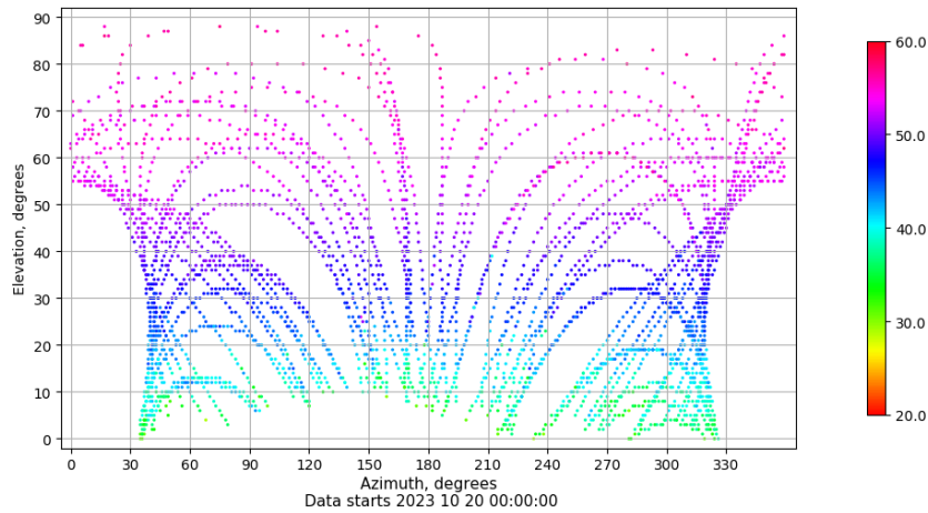
Azimuth-elevation plot for station LPAL. Signal to Noise S1C Data file LPAL00ESP_R_2023293.xtr
