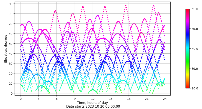
Time-elevation plot for station LPAL. Signal to Noise S1C Data file LPAL00ESP_R_2023293.xtr
