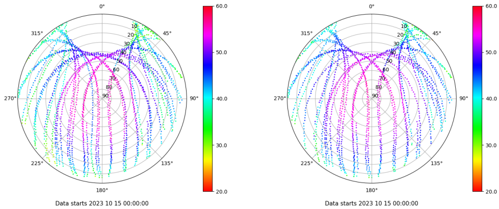
Skyplot for station LPAL. Signal to Noise S1C Data file LPAL00ESP_R_2023288.xtr Skyplot for station LPAL. Signal to Noise S2C Data file LPAL00ESP_R_2023288.xtr
