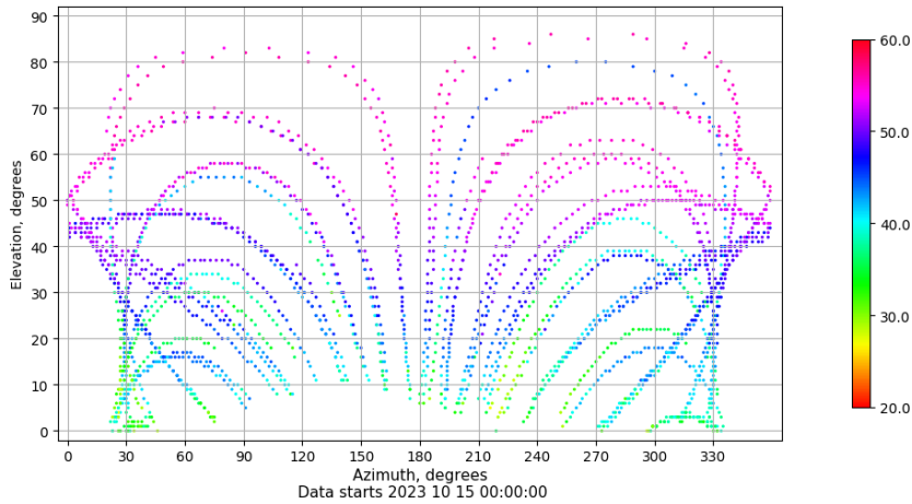
Azimuth-elevation plot for station LPAL. Signal to Noise S1C Data file LPAL00ESP_R_2023288.xtr
