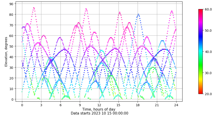
Time-elevation plot for station LPAL. Signal to Noise S1C Data file LPAL00ESP_R_2023288.xtr
