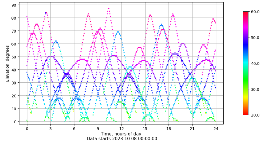
Time-elevation plot for station LPAL. Signal to Noise S1C Data file LPAL00ESP_R_2023281.xtr
