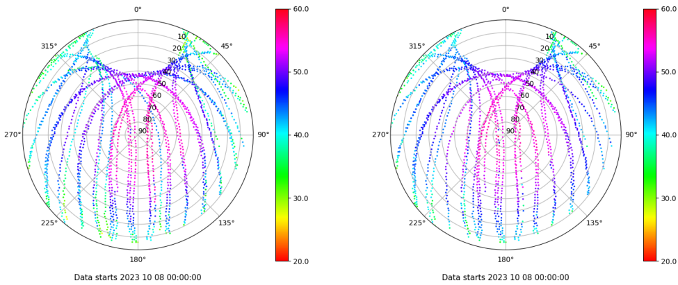
Skyplot for station LPAL. Signal to Noise S1C Data file LPAL00ESP_R_2023281.xtr Skyplot for station LPAL. Signal to Noise S2C Data file LPAL00ESP_R_2023281.xtr
