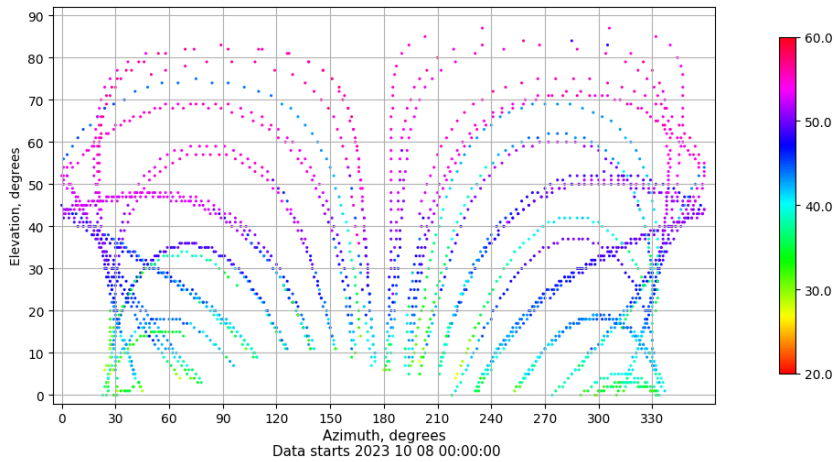
Azimuth-elevation plot for station LPAL. Signal to Noise S1C Data file LPAL00ESP_R_2023281.xtr
