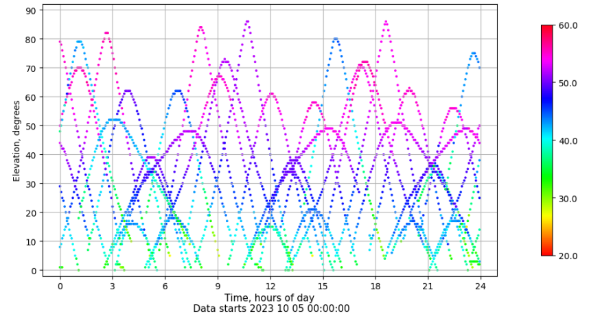
Time-elevation plot for station LPAL. Signal to Noise S1C Data file LPAL00ESP_R_2023278.xtr
