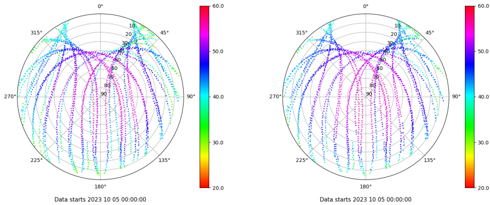
Skyplot for station LPAL. Signal to Noise S1C Data file LPAL00ESP_R_2023278.xtr Skyplot for station LPAL. Signal to Noise S2C Data file LPAL00ESP_R_2023278.xtr
