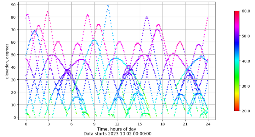
Time-elevation plot for station LPAL. Signal to Noise S1C Data file LPAL00ESP_R_2023275.xtr
