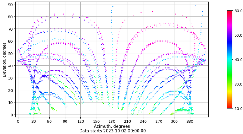
Azimuth-elevation plot for station LPAL. Signal to Noise S1C Data file LPAL00ESP_R_2023275.xtr
