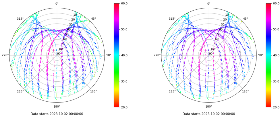
Skyplot for station LPAL. Signal to Noise S1C Data file LPAL00ESP_R_2023275.xtr Skyplot for station LPAL. Signal to Noise S2C Data file LPAL00ESP_R_2023275.xtr
