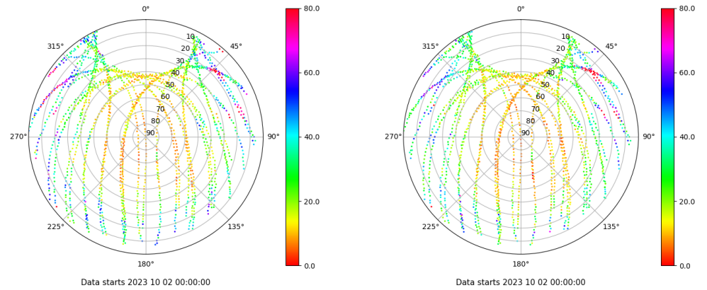
Skyplot for station LPAL. Parameter M1C Data file LPAL00ESP_R_2023275.xtr Skyplot for station LPAL. Parameter M2C Data file LPAL00ESP_R_2023275.xtr
