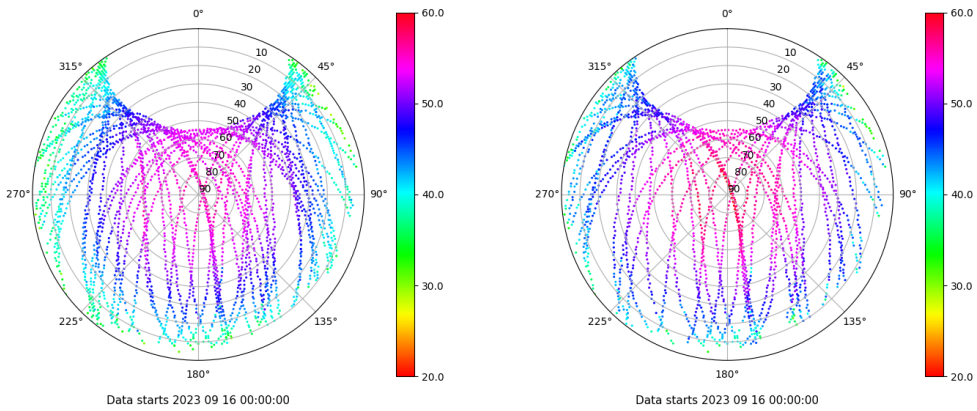
Skyplot for station LPAL. Signal to Noise S1C Data file LPAL00ESP_R_2023259.xtr Skyplot for station LPAL. Signal to Noise S2S Data file LPAL00ESP_R_2023259.xtr
