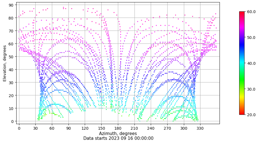
Azimuth-elevation plot for station LPAL. Signal to Noise S1C Data file LPAL00ESP_R_2023259.xtr
