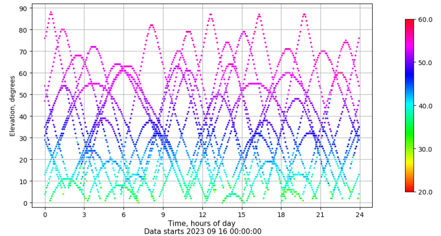
Time-elevation plot for station LPAL. Signal to Noise S1C Data file LPAL00ESP_R_2023259.xtr
