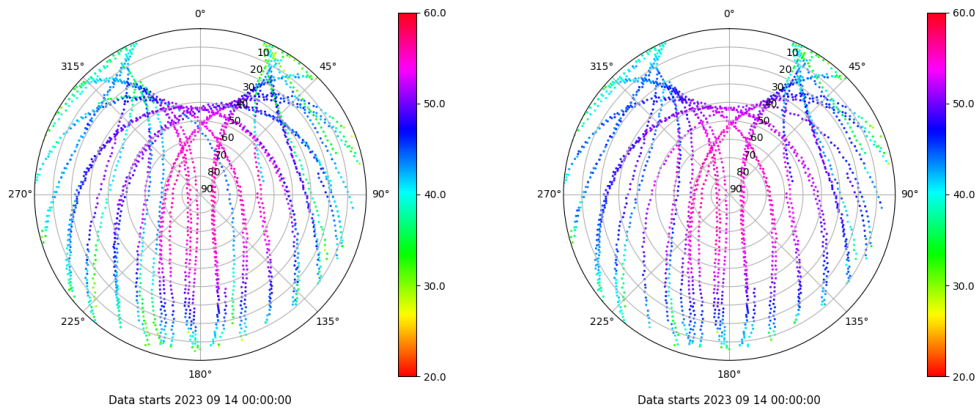
Skyplot for station LPAL. Signal to Noise S1C Data file LPAL00ESP_R_2023257.xtr Skyplot for station LPAL. Signal to Noise S2C Data file LPAL00ESP_R_2023257.xtr
