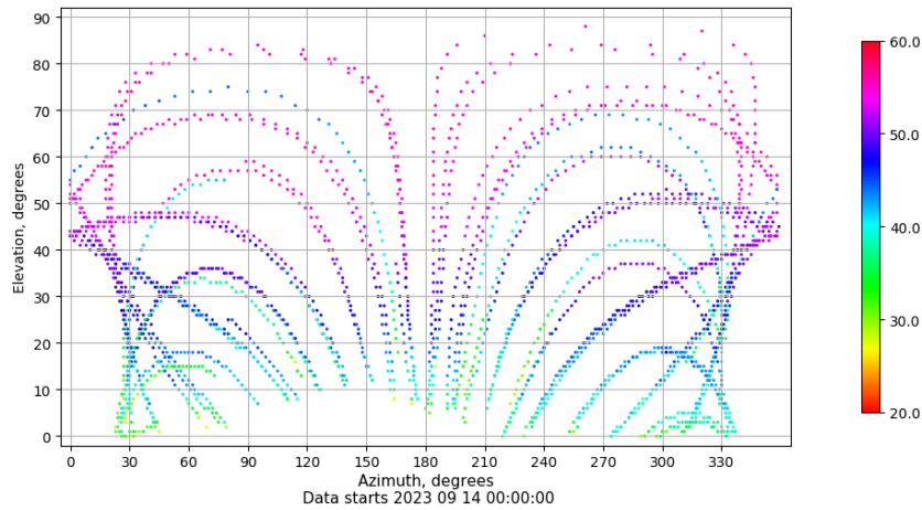
Azimuth-elevation plot for station LPAL. Signal to Noise S1C Data file LPAL00ESP_R_2023257.xtr
