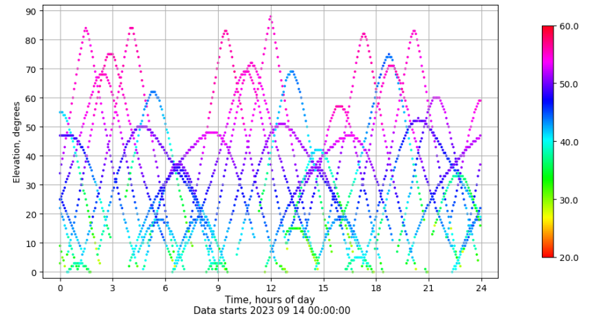
Time-elevation plot for station LPAL. Signal to Noise S1C Data file LPAL00ESP_R_2023257.xtr
