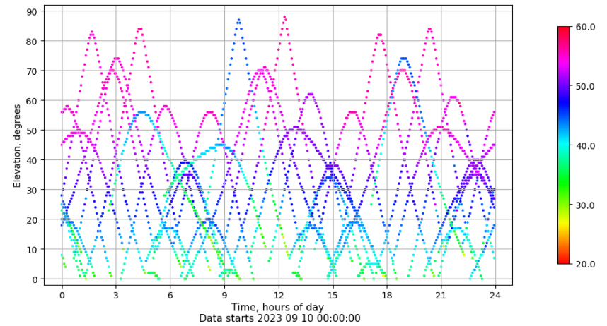
Time-elevation plot for station LPAL. Signal to Noise S1C Data file LPAL00ESP_R_2023253.xtr
