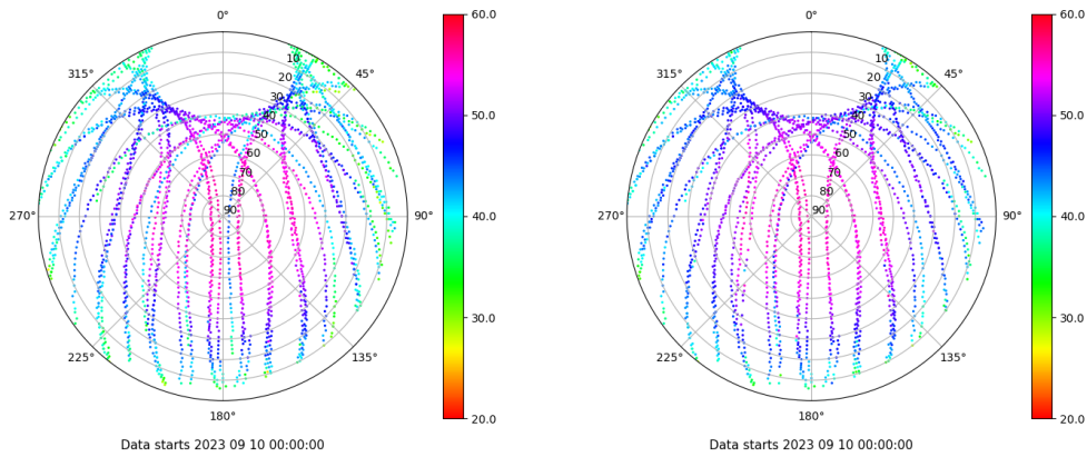
Skyplot for station LPAL. Signal to Noise S1C Data file LPAL00ESP_R_2023253.xtr Skyplot for station LPAL. Signal to Noise S2C Data file LPAL00ESP_R_2023253.xtr
