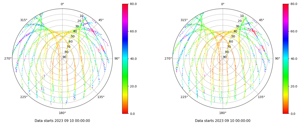
Skyplot for station LPAL. Parameter M1C Data file LPAL00ESP_R_2023253.xtr Skyplot for station LPAL. Parameter M2C Data file LPAL00ESP_R_2023253.xtr
