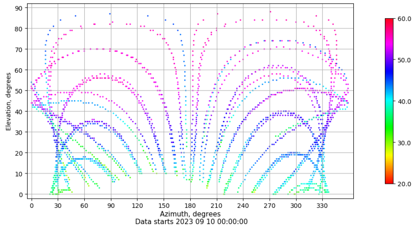
Azimuth-elevation plot for station LPAL. Signal to Noise S1C Data file LPAL00ESP_R_2023253.xtr
