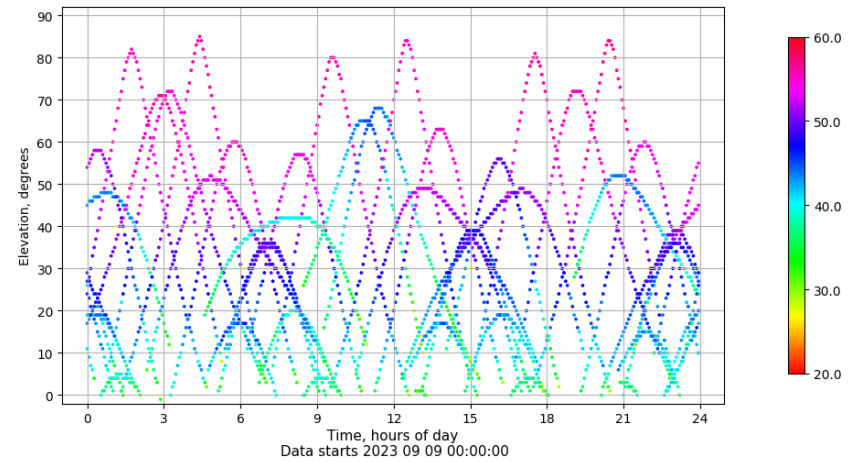
Time-elevation plot for station LPAL. Signal to Noise S1C Data file LPAL00ESP_R_2023252.xtr
