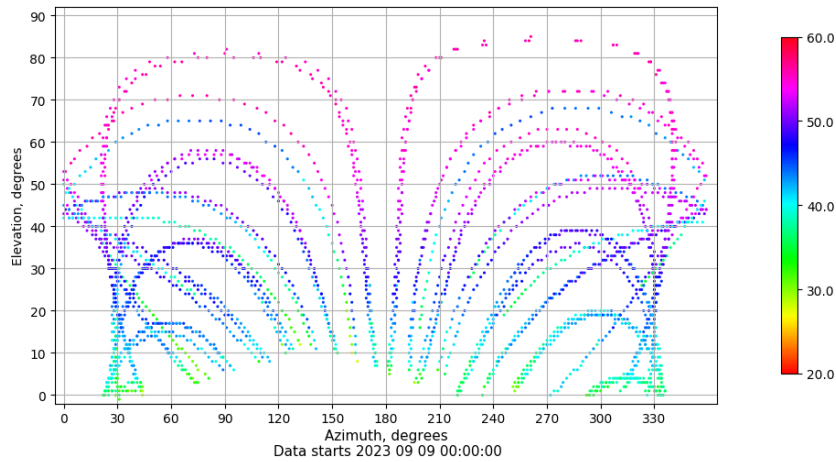
Azimuth-elevation plot for station LPAL. Signal to Noise S1C Data file LPAL00ESP_R_2023252.xtr
