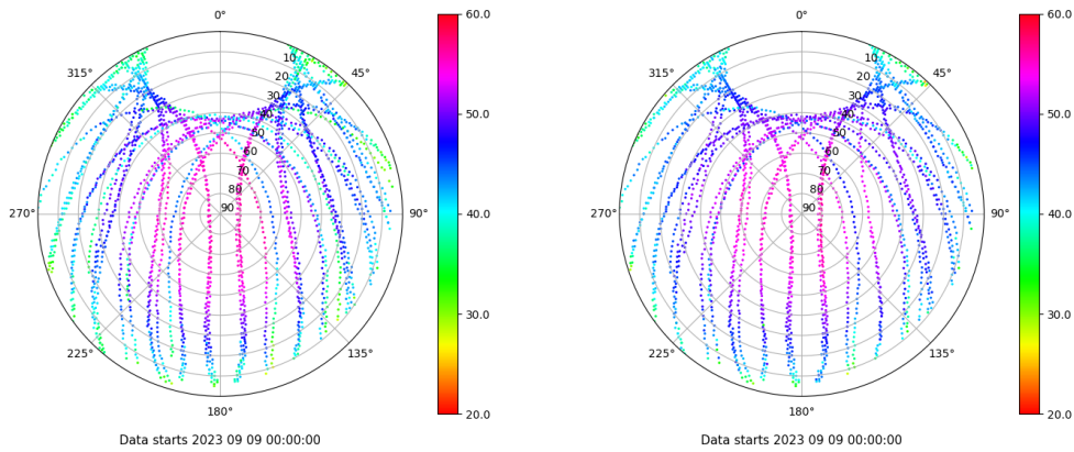
Skyplot for station LPAL. Signal to Noise S1C Data file LPAL00ESP_R_2023252.xtr Skyplot for station LPAL. Signal to Noise S2C Data file LPAL00ESP_R_2023252.xtr
