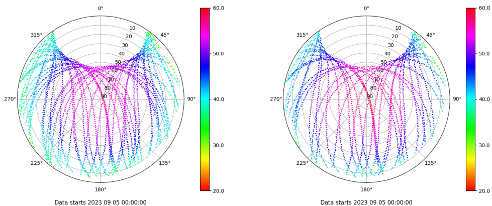
Skyplot for station LPAL. Signal to Noise S1C Data file LPAL00ESP_R_2023248.xtr Skyplot for station LPAL. Signal to Noise S2S Data file LPAL00ESP_R_2023248.xtr
