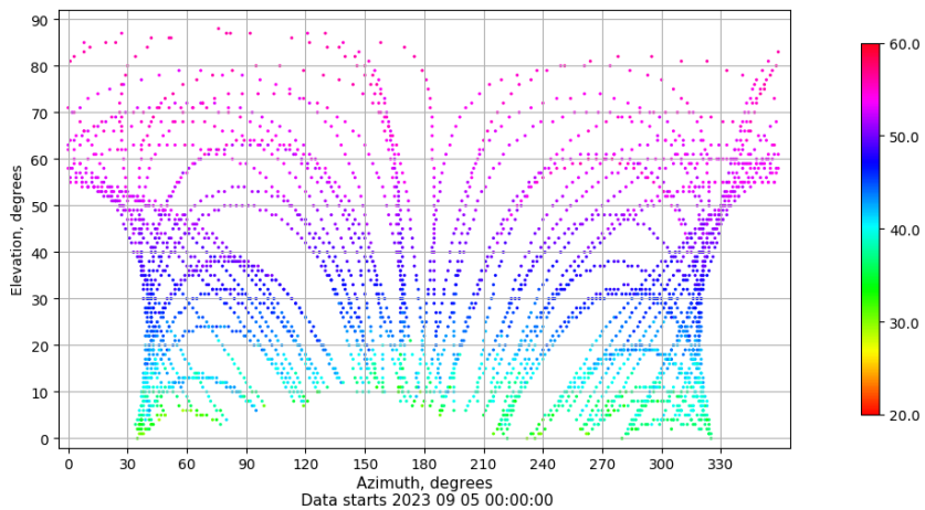
Azimuth-elevation plot for station LPAL. Signal to Noise S1C Data file LPAL00ESP_R_2023248.xtr
