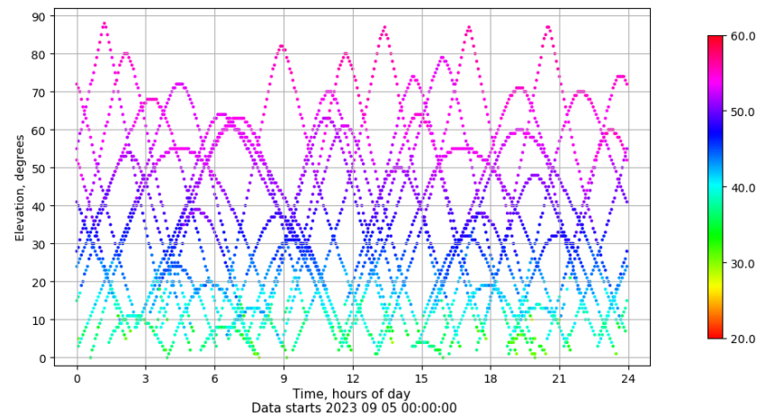
Time-elevation plot for station LPAL. Signal to Noise S1C Data file LPAL00ESP_R_2023248.xtr
