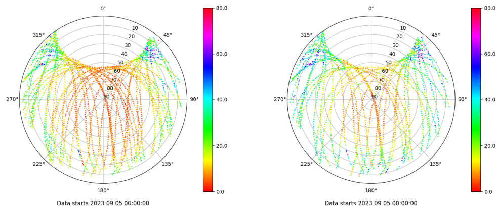
Skyplot for station LPAL. Parameter M1C Data file LPAL00ESP_R_2023248.xtr Skyplot for station LPAL. Parameter M2S Data file LPAL00ESP_R_2023248.xtr
