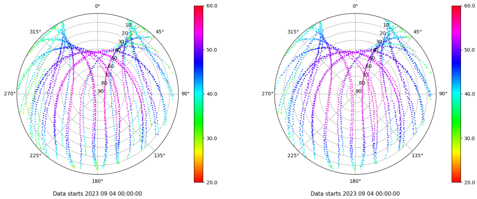
Skyplot for station LPAL. Signal to Noise S1C Data file LPAL00ESP_R_2023247.xtr Skyplot for station LPAL. Signal to Noise S2C Data file LPAL00ESP_R_2023247.xtr
