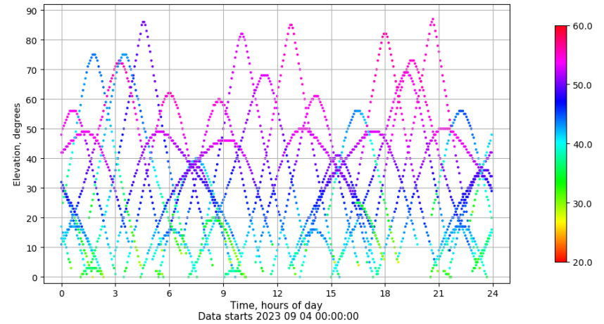
Time-elevation plot for station LPAL. Signal to Noise S1C Data file LPAL00ESP_R_2023247.xtr
