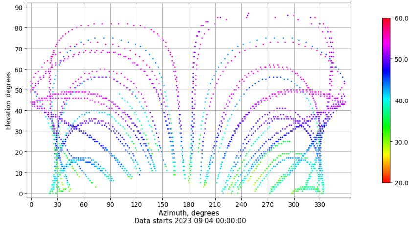
Azimuth-elevation plot for station LPAL. Signal to Noise S1C Data file LPAL00ESP_R_2023247.xtr
