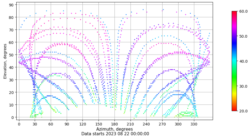
Azimuth-elevation plot for station LPAL. Signal to Noise S1C Data file LPAL00ESP_R_2023234.xtr
