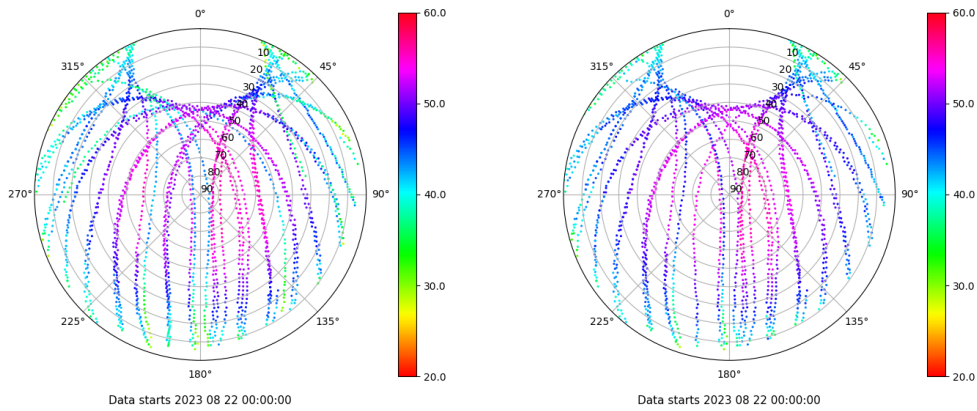
Skyplot for station LPAL. Signal to Noise S1C Data file LPAL00ESP_R_2023234.xtr Skyplot for station LPAL. Signal to Noise S2C Data file LPAL00ESP_R_2023234.xtr
