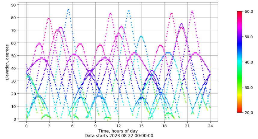
Time-elevation plot for station LPAL. Signal to Noise S1C Data file LPAL00ESP_R_2023234.xtr
