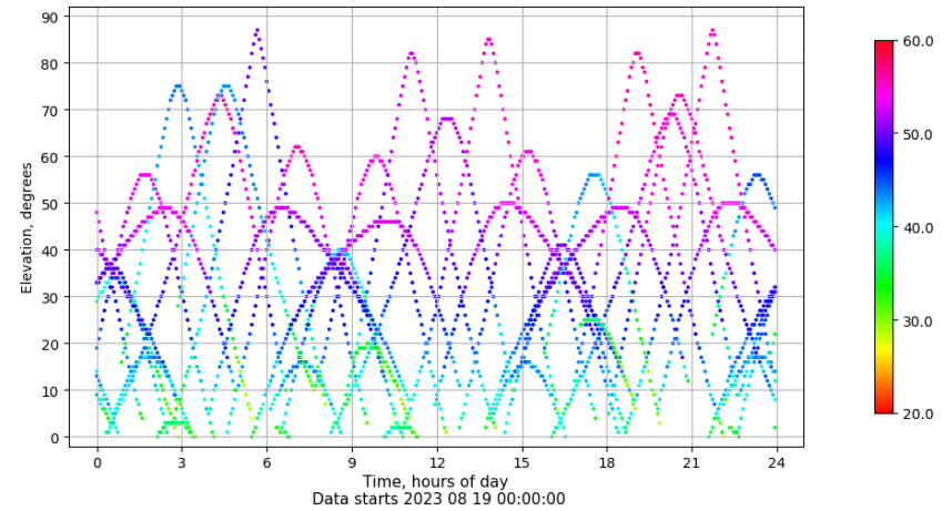
Time-elevation plot for station LPAL. Signal to Noise S1C Data file LPAL00ESP_R_2023231.xtr
