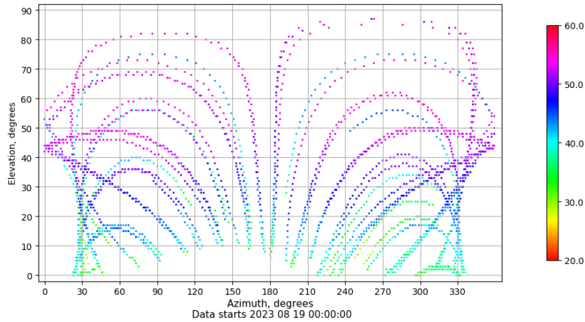
Azimuth-elevation plot for station LPAL. Signal to Noise S1C Data file LPAL00ESP_R_2023231.xtr
