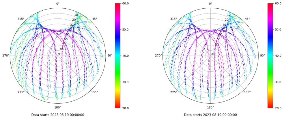
Skyplot for station LPAL. Signal to Noise S1C Data file LPAL00ESP_R_2023231.xtr Skyplot for station LPAL. Signal to Noise S2C Data file LPAL00ESP_R_2023231.xtr
