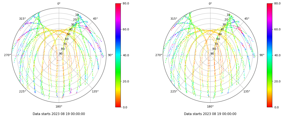
Skyplot for station LPAL. Parameter M1C Data file LPAL00ESP_R_2023231.xtr Skyplot for station LPAL. Parameter M2C Data file LPAL00ESP_R_2023231.xtr
