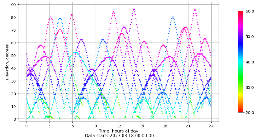
Time-elevation plot for station LPAL. Signal to Noise S1C Data file LPAL00ESP_R_2023230.xtr
