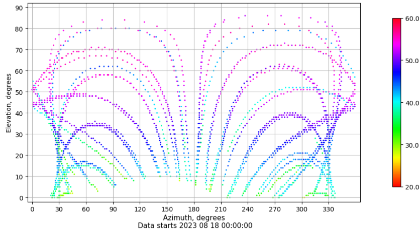
Azimuth-elevation plot for station LPAL. Signal to Noise S1C Data file LPAL00ESP_R_2023230.xtr
