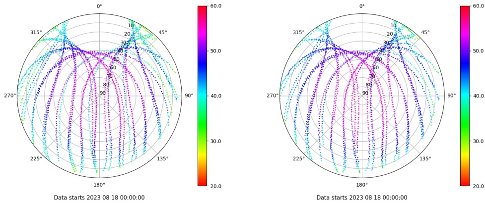
Skyplot for station LPAL. Signal to Noise S1C Data file LPAL00ESP_R_2023230.xtr Skyplot for station LPAL. Signal to Noise S2C Data file LPAL00ESP_R_2023230.xtr
