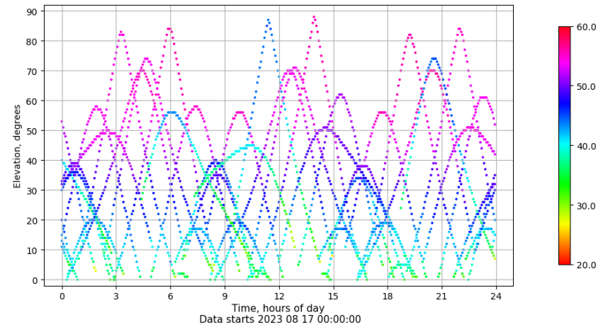
Time-elevation plot for station LPAL. Signal to Noise S1C Data file LPAL00ESP_R_2023229.xtr
