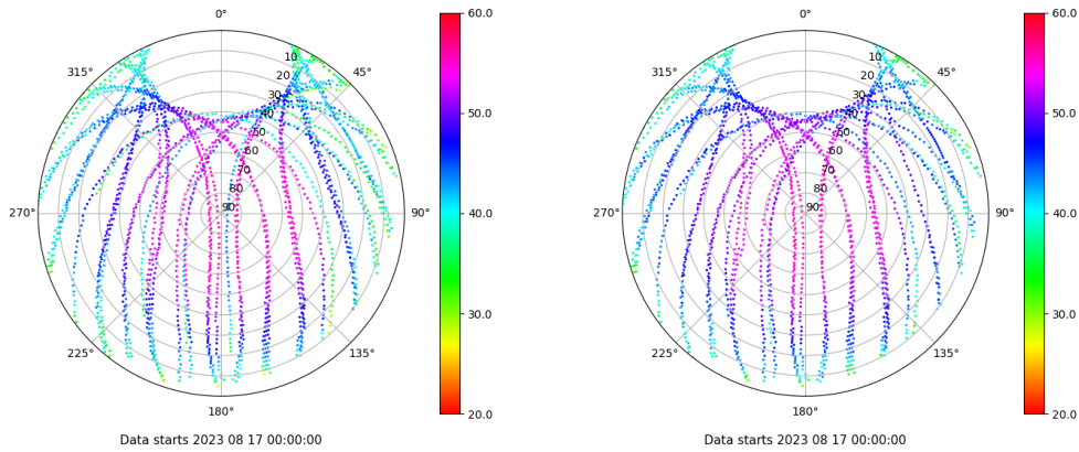
Skyplot for station LPAL. Signal to Noise S1C Data file LPAL00ESP_R_2023229.xtr Skyplot for station LPAL. Signal to Noise S2C Data file LPAL00ESP_R_2023229.xtr
