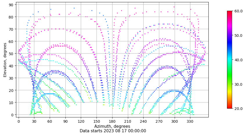
Azimuth-elevation plot for station LPAL. Signal to Noise S1C Data file LPAL00ESP_R_2023229.xtr
