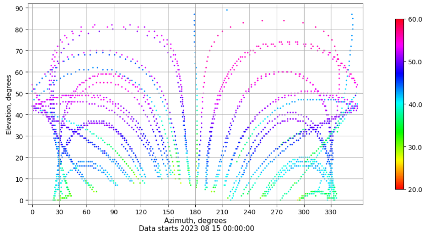
Azimuth-elevation plot for station LPAL. Signal to Noise S1C Data file LPAL00ESP_R_2023227.xtr
