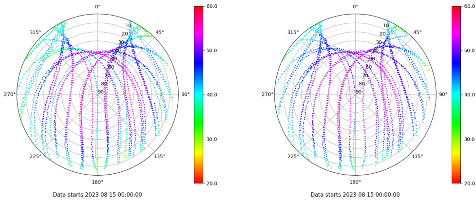
Skyplot for station LPAL. Signal to Noise S1C Data file LPAL00ESP_R_2023227.xtr Skyplot for station LPAL. Signal to Noise S2C Data file LPAL00ESP_R_2023227.xtr
